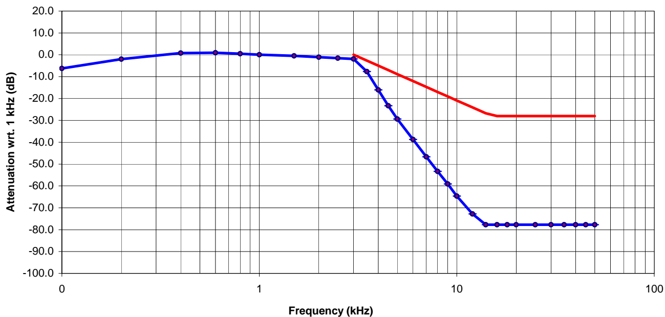
Audio Frequency Response 25 kHz Channel Spacing
