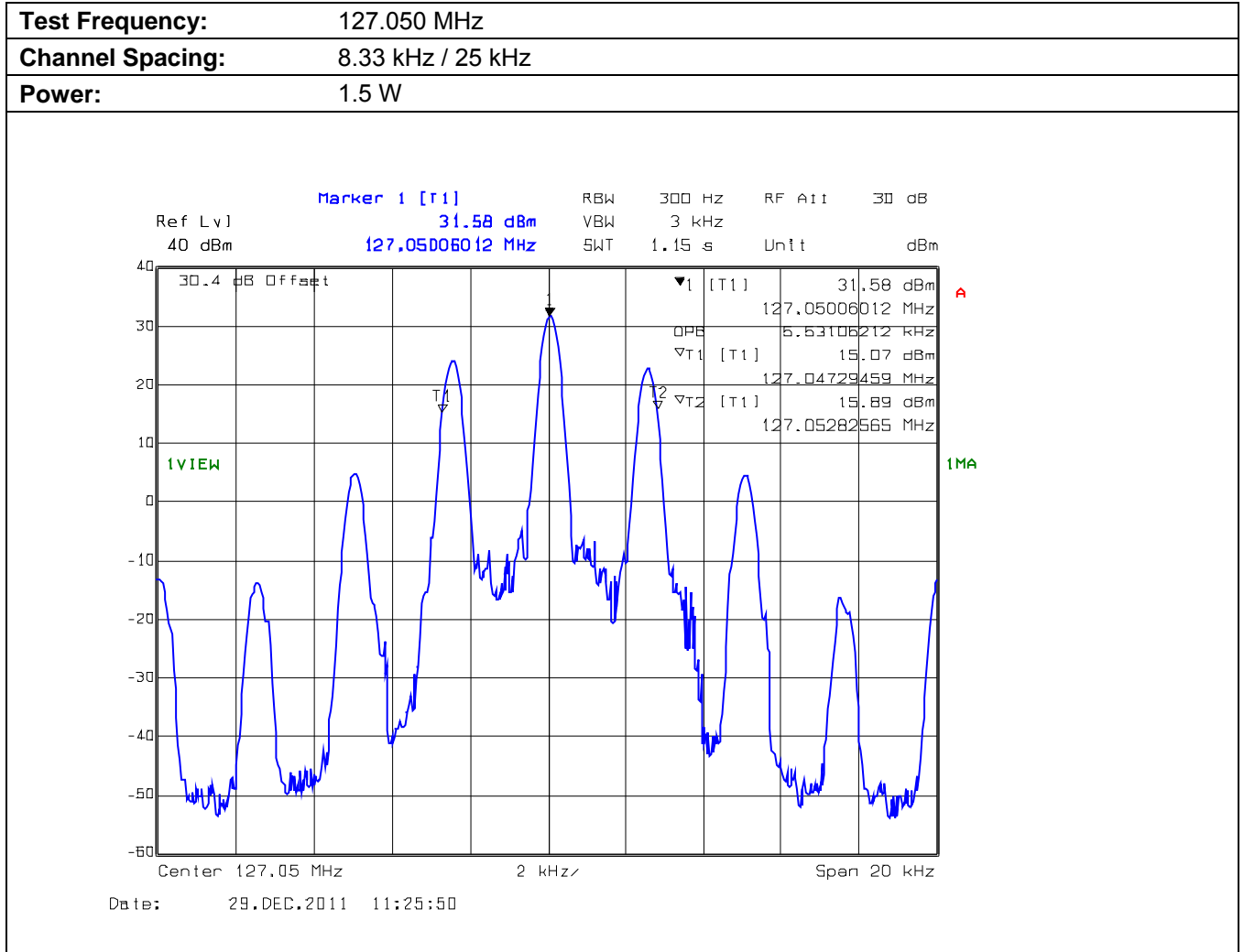
Plot 5.6.4.1.2. Occupied Bandwidth for 127.050 MHz
