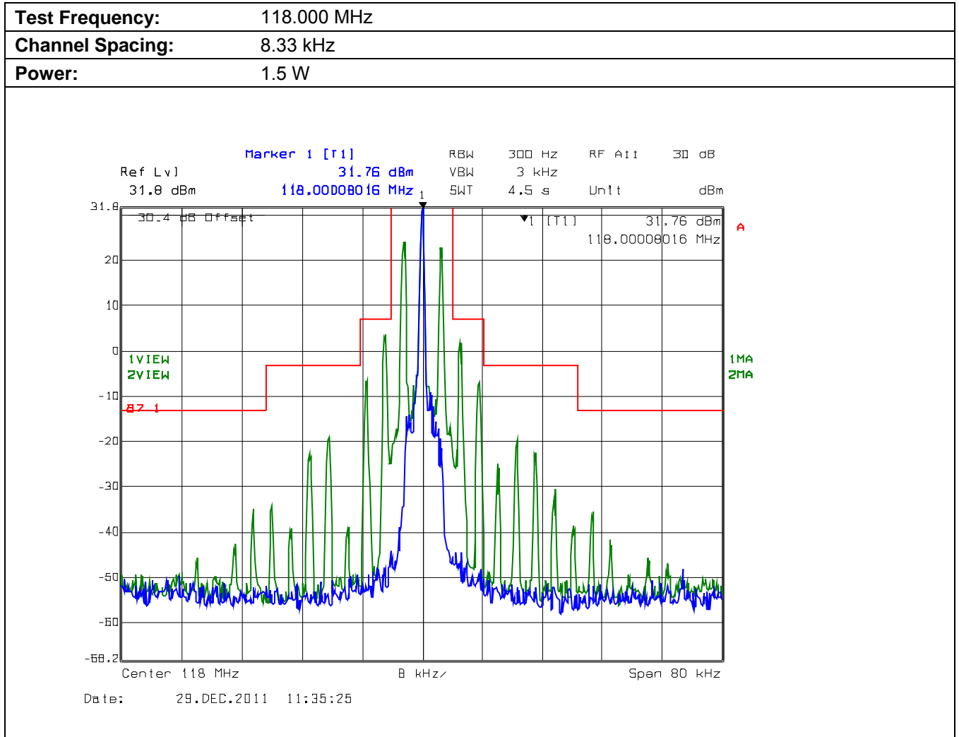
Plot 5.6.4.2.1. Emission Limitation for 118.000 MHz
