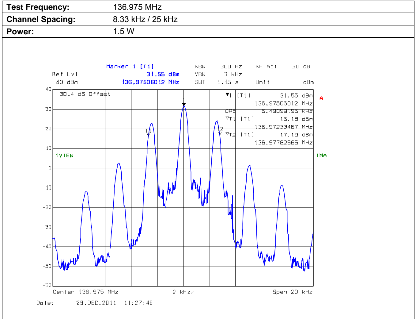
Plot 5.6.4.1.3. Occupied Bandwidth for 136.975 MHz
