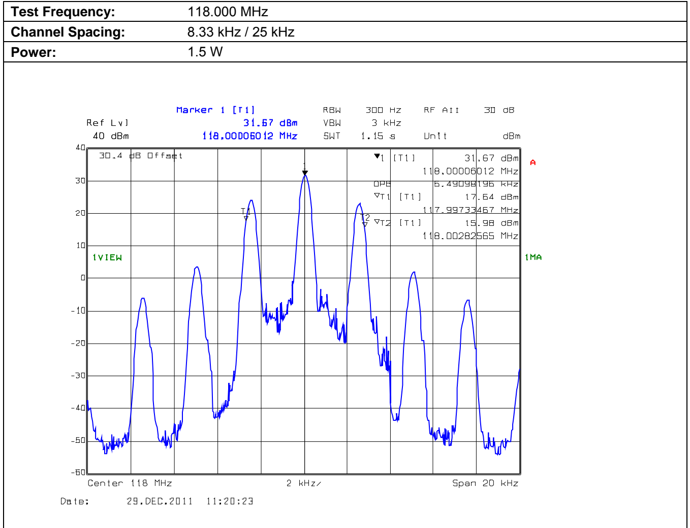
Plot 5.6.4.1.1. Occupied Bandwidth for 118.000 MHz
