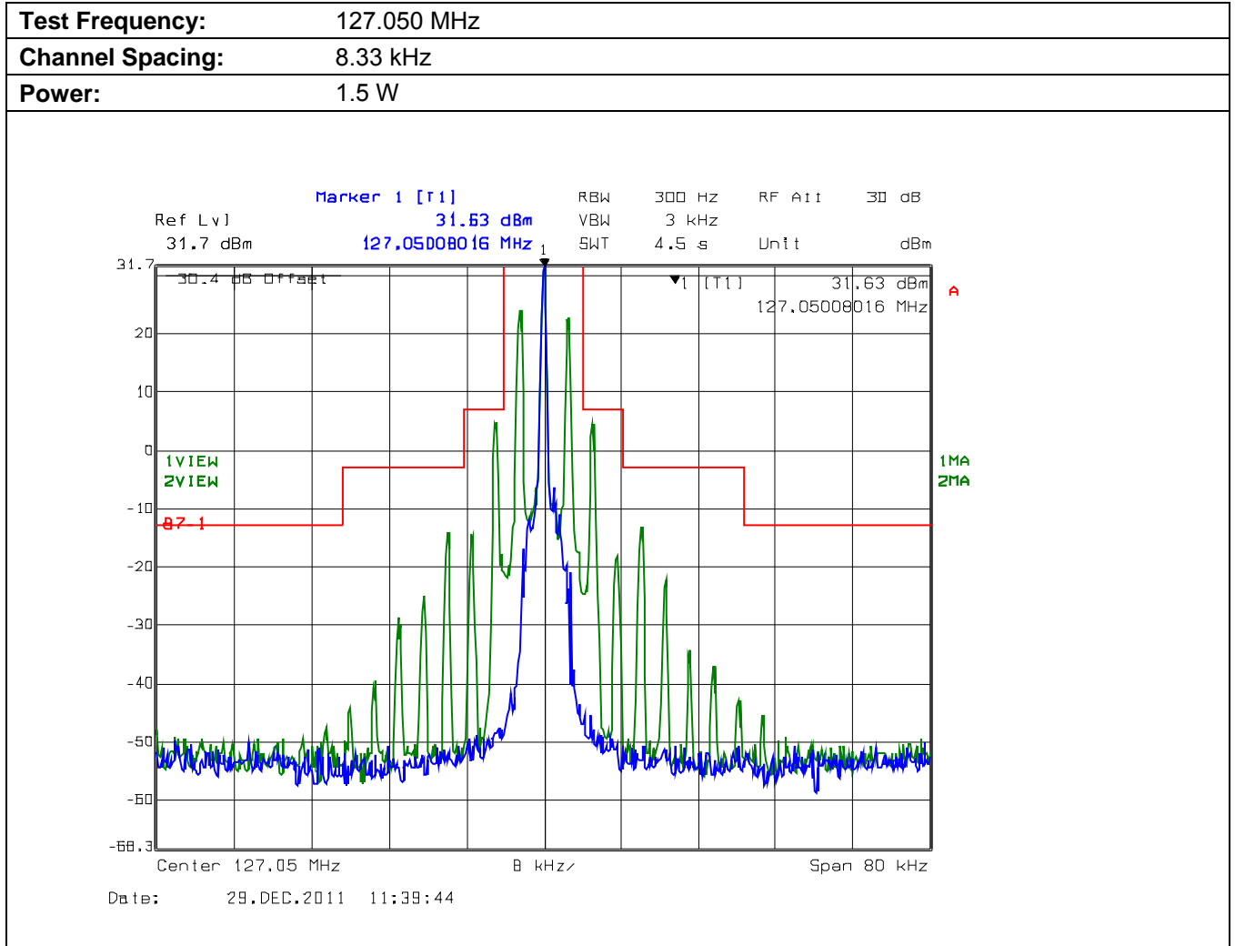
Plot 5.6.4.2.2. Emission Limitation for 127.050 MHz
