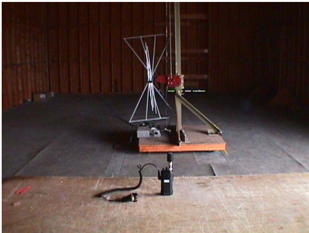
Radiated Emissions Orthogonal Position #1
