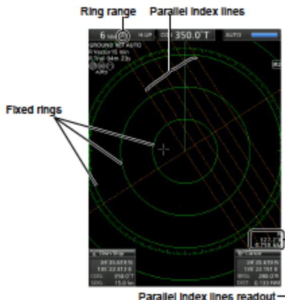
Parallel Index lines readout
