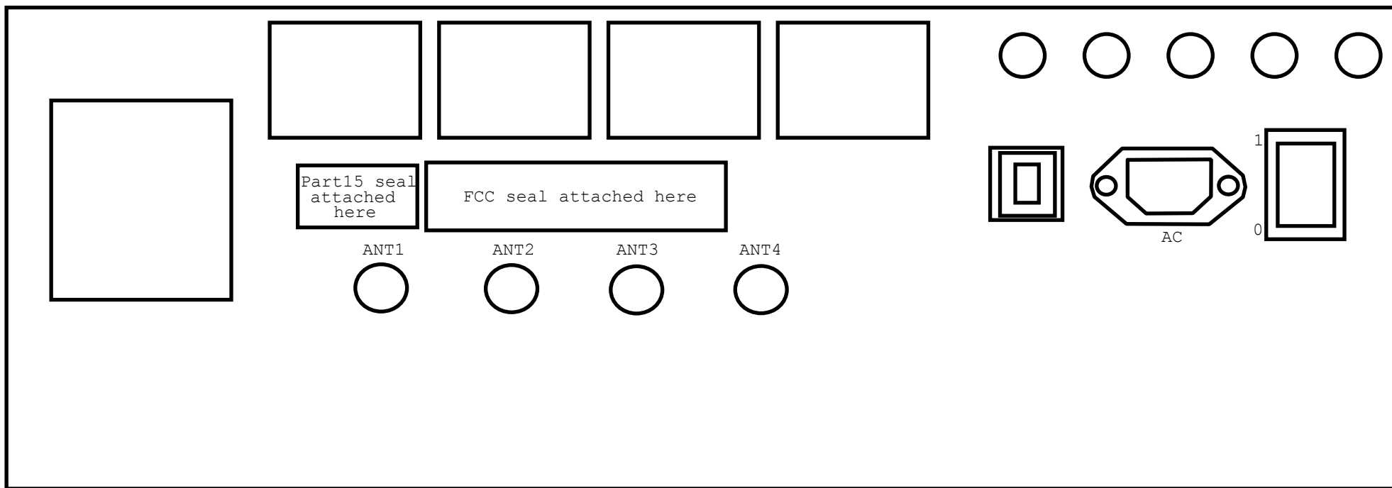
REAR VIEW OF IC-7800
