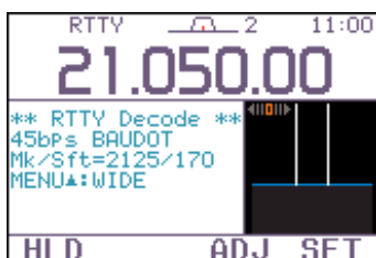
RTTY tuning meter
