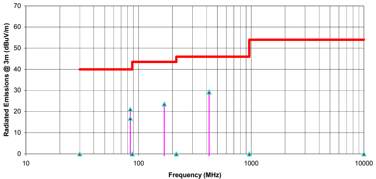
Radiated Emissions Measurements @ 3m OFTS Icom Scanning Receiver, Model IC-706MKIIG Receiver Frequency: 100 MHz in 0.03-200 MHz Band at ANT 1 and ANT 2 Ports
