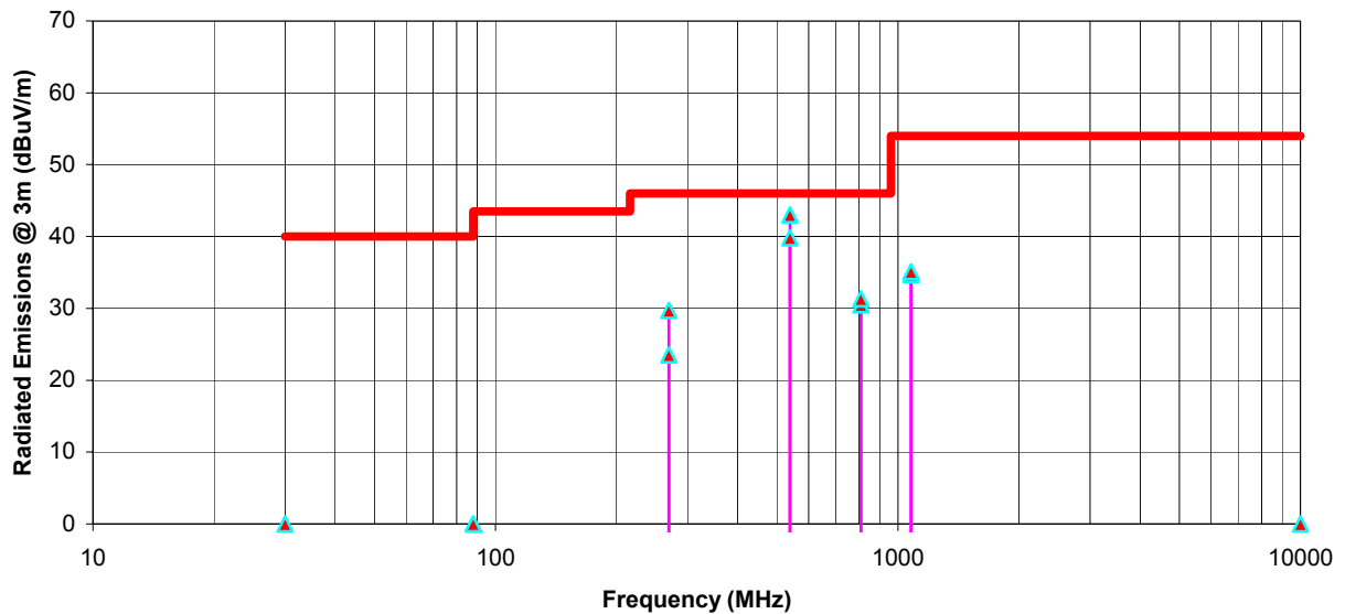
Radiated Emissions Measurements @ 3m OFTS Icom Scanning Receiver, Model IC-706MKIIG Receiver Frequency: 470 MHz in 400-470 MHz Band at ANT 1 and ANT 2 Ports
