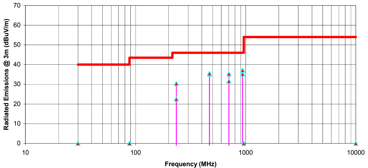
Radiated Emissions Measurements @ 3m OFTS Icom Scanning Receiver, Model IC-706MKIIG Receiver Frequency: 400 MHz in 400-470 MHz Band at ANT 1 and ANT 2 Ports
