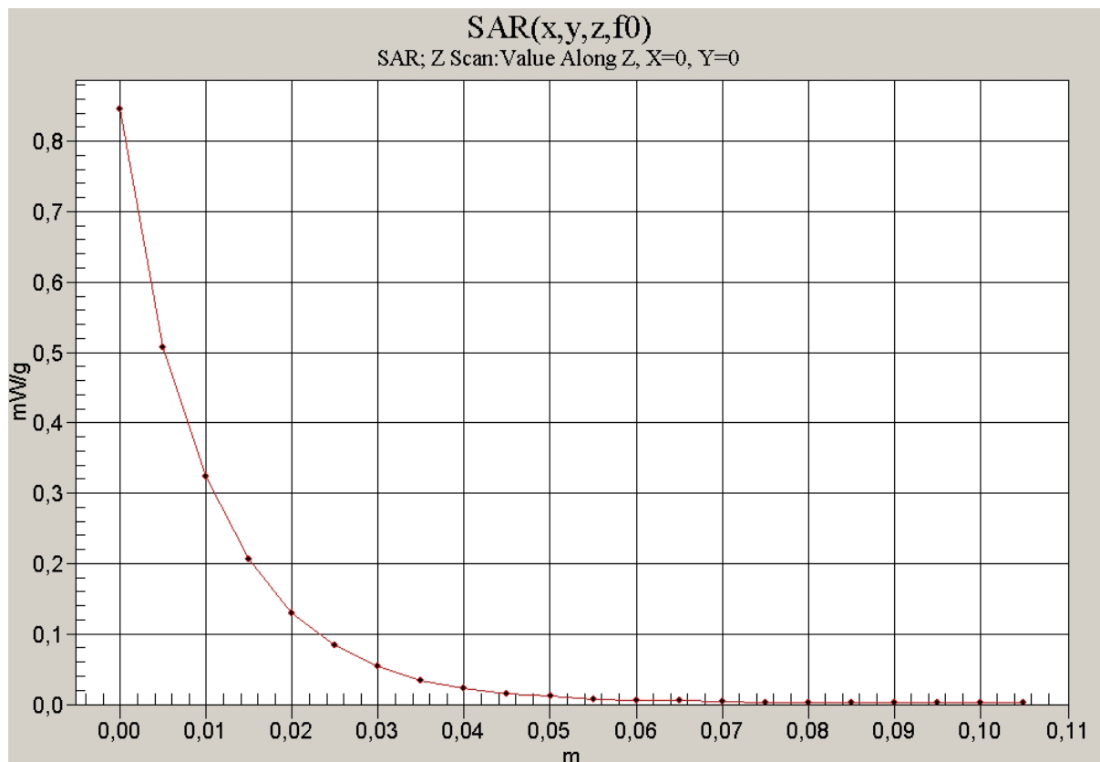
Z-Axis-Scan 1900 MHz head
