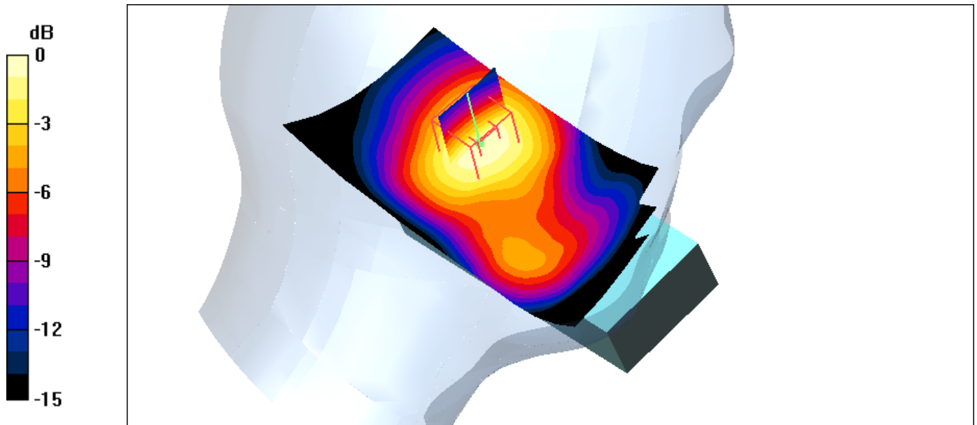
0 dB = 0.442mW/g
