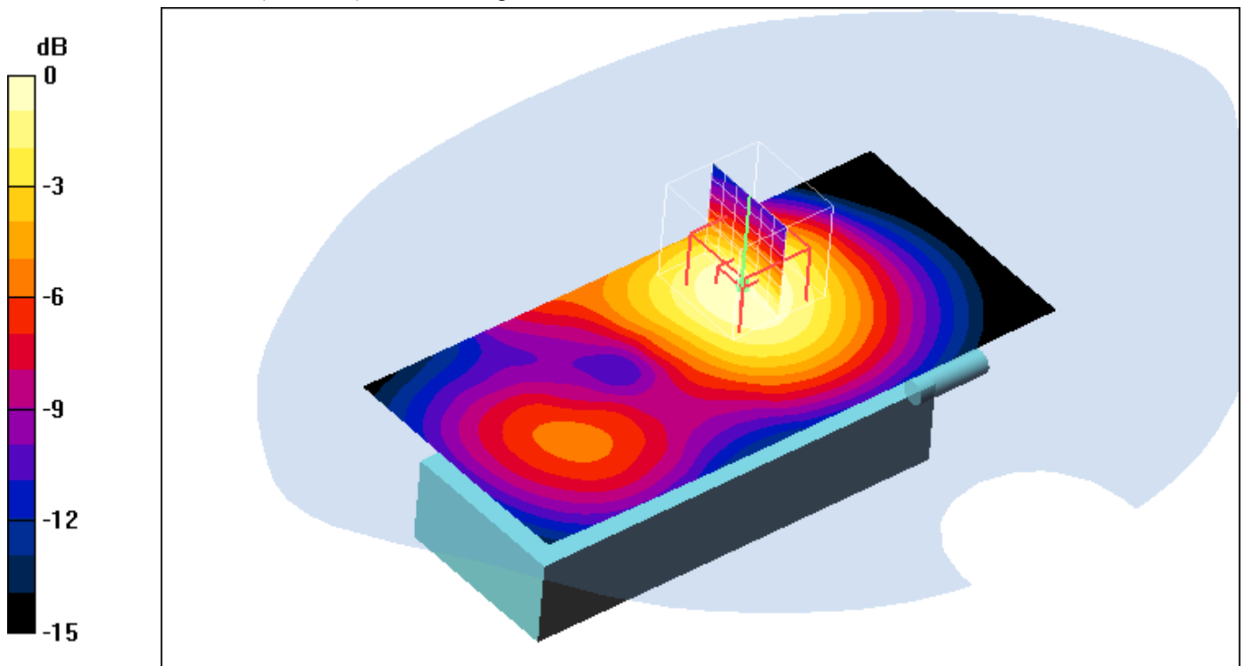
0 dB = 0.576mW/g
