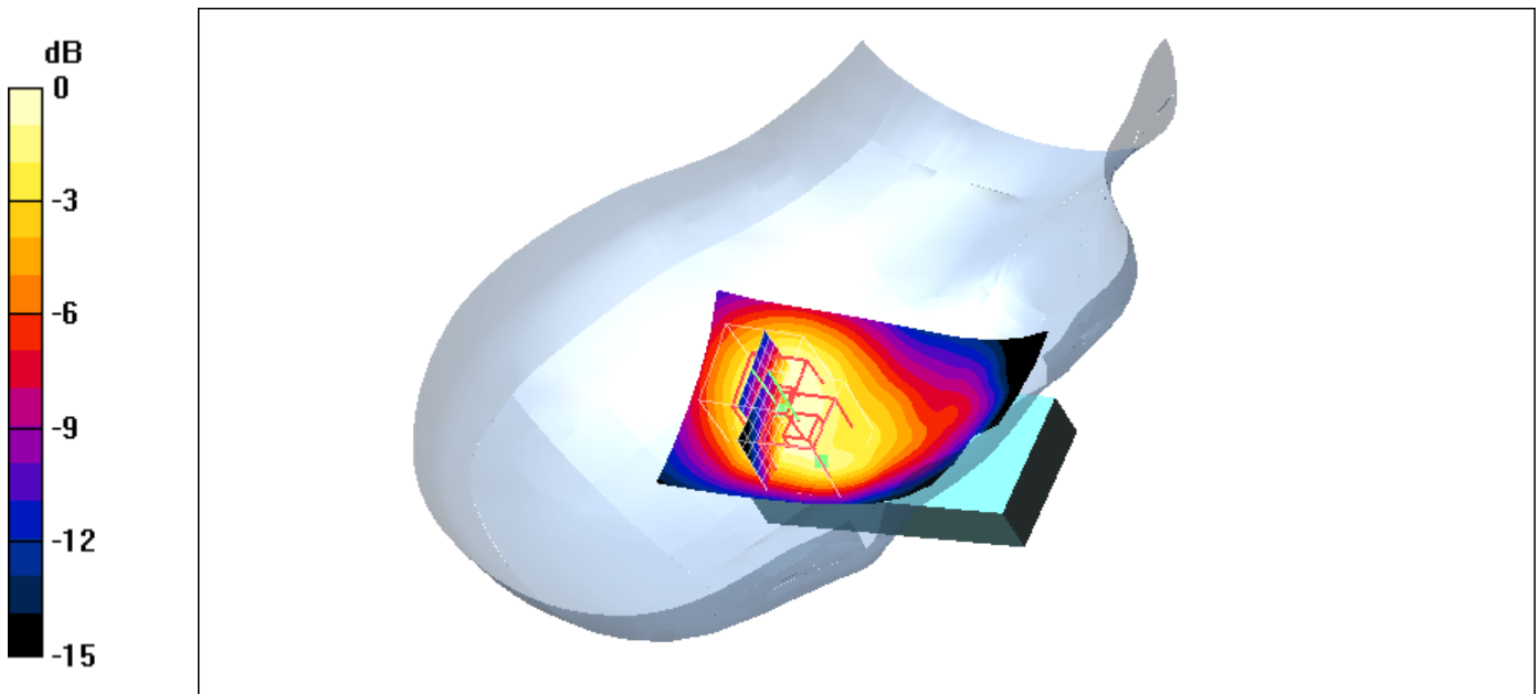
0 dB = 0.483mW/g
