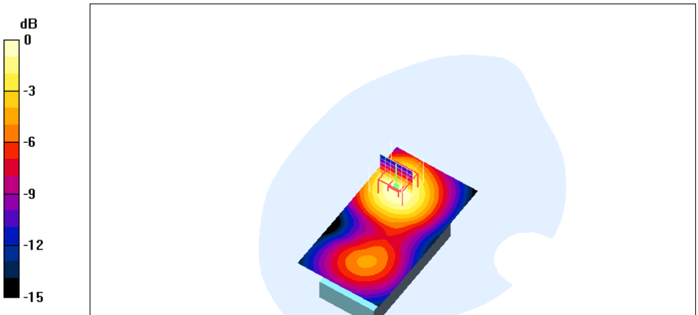
0 dB = 0.740mW/g
