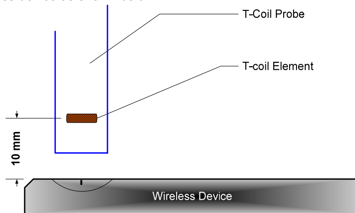
Figure 5-11 Measurement Distance
