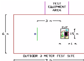
Figure 3-2. Dimensions of Outdoor Test Site
