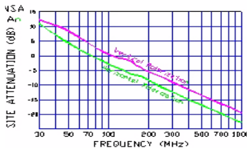
Figure 3-4. Normalized Site Attenuation Curves (H&V)
