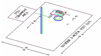
Figure 3-3. Turntable and System Setup
