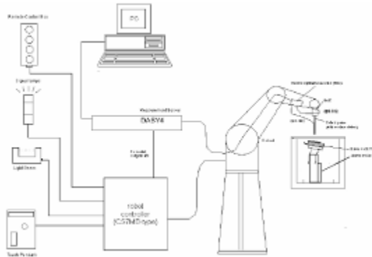
Figure 5-6 SPEAG Robotic System Diagram
