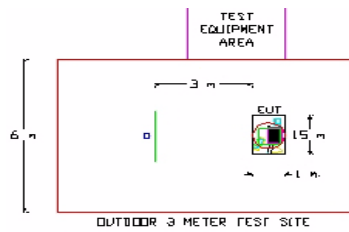
Figure 3-2. Dimensions of Outdoor Test Site
