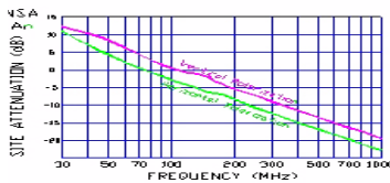
Figure 3-4. Normalized Site Attenuation Curves (H&V)
