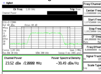
Figure 20 Signal Generator Modulated Signal
