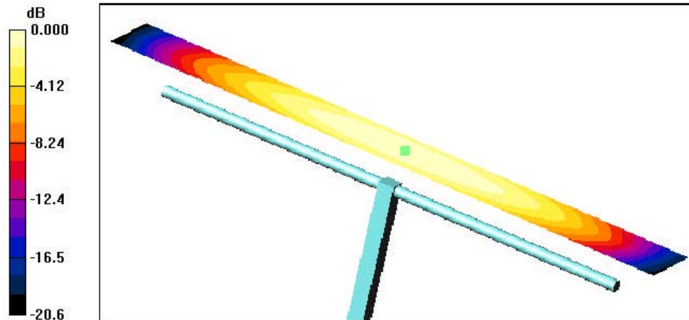
0 dB = 0.511A/m
