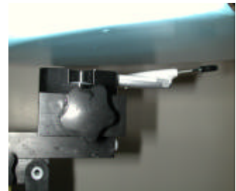
Figure 18. PCS Body SAR Test Setup
