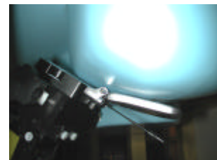
Figure 17. AMPS Head SAR Test Setup
