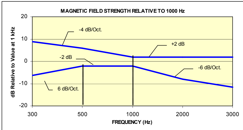
Figure 4-1 Magnetic field frequency response for Wireless Devices with an axial field between -10\text{ dB} to -13\text{ dB (A/m)} at 1 kHz
