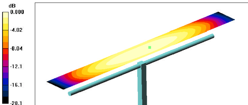
0 dB = 0.485A/m
