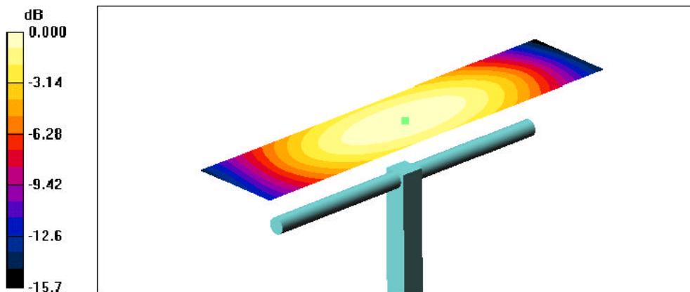
0 dB = 0.446A/m
