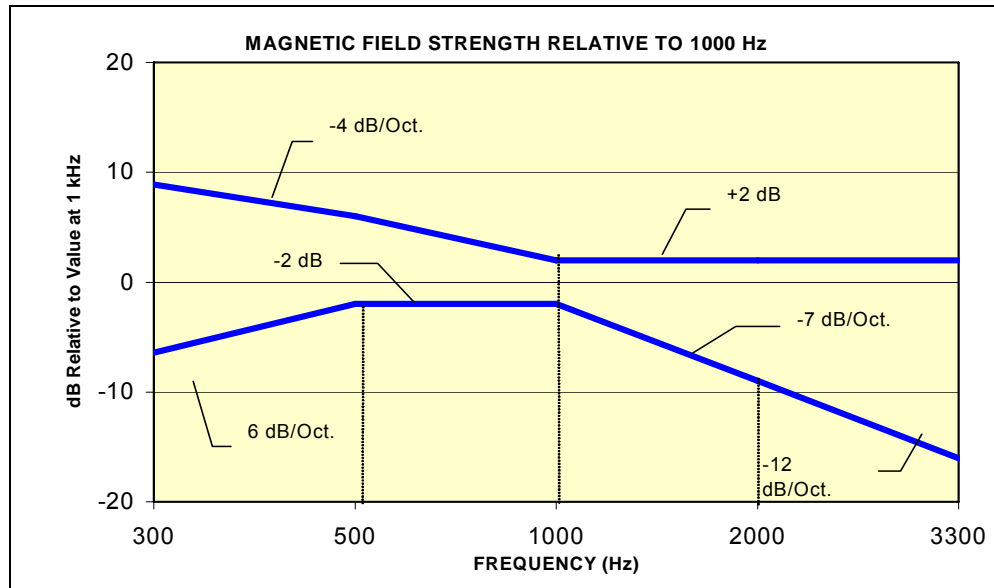
Figure 4-2 Magnetic Field frequency response for wireless devices with an axial field that exceeds -10 dB(A/m) at 1 kHz
