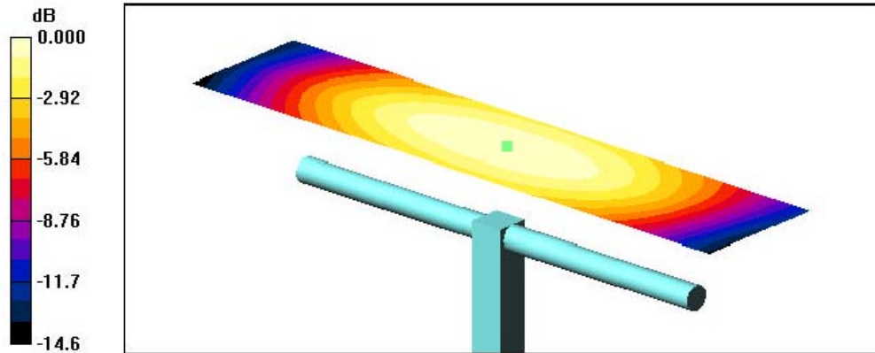
0 dB = 0.431A/m
