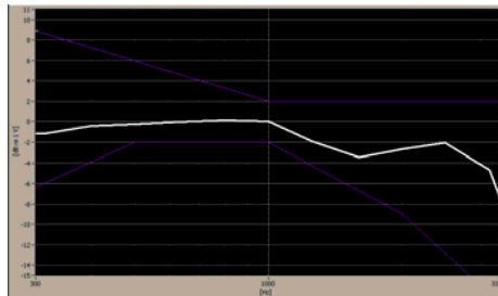
Figure 6-1 Axial Frequency Response
