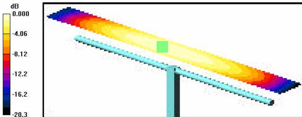
0 dB = 0.465A/m
