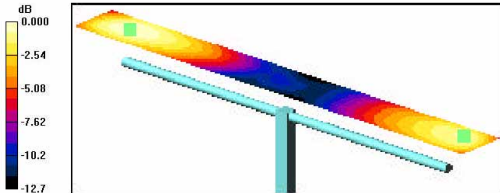
0 dB = 176.6V/m
