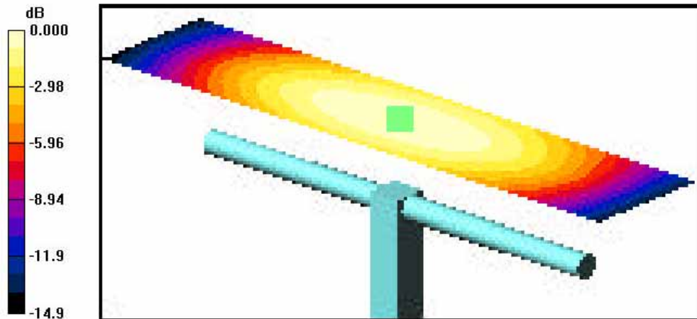
0 dB = 0.446A/m
