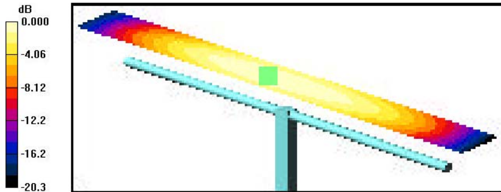
0 dB = 0.465A/m
