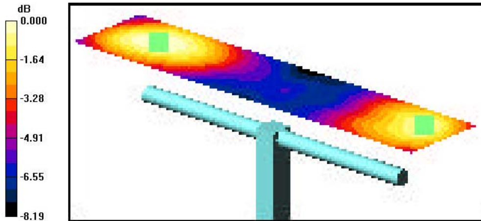
0 dB = 152.1V/m
