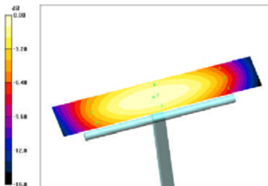
0 dB = 0.430A/m
