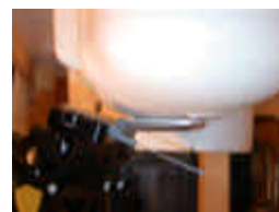
Figure 14.11 Left Head SAR Test Setup -- Cheek / Touch Position --
