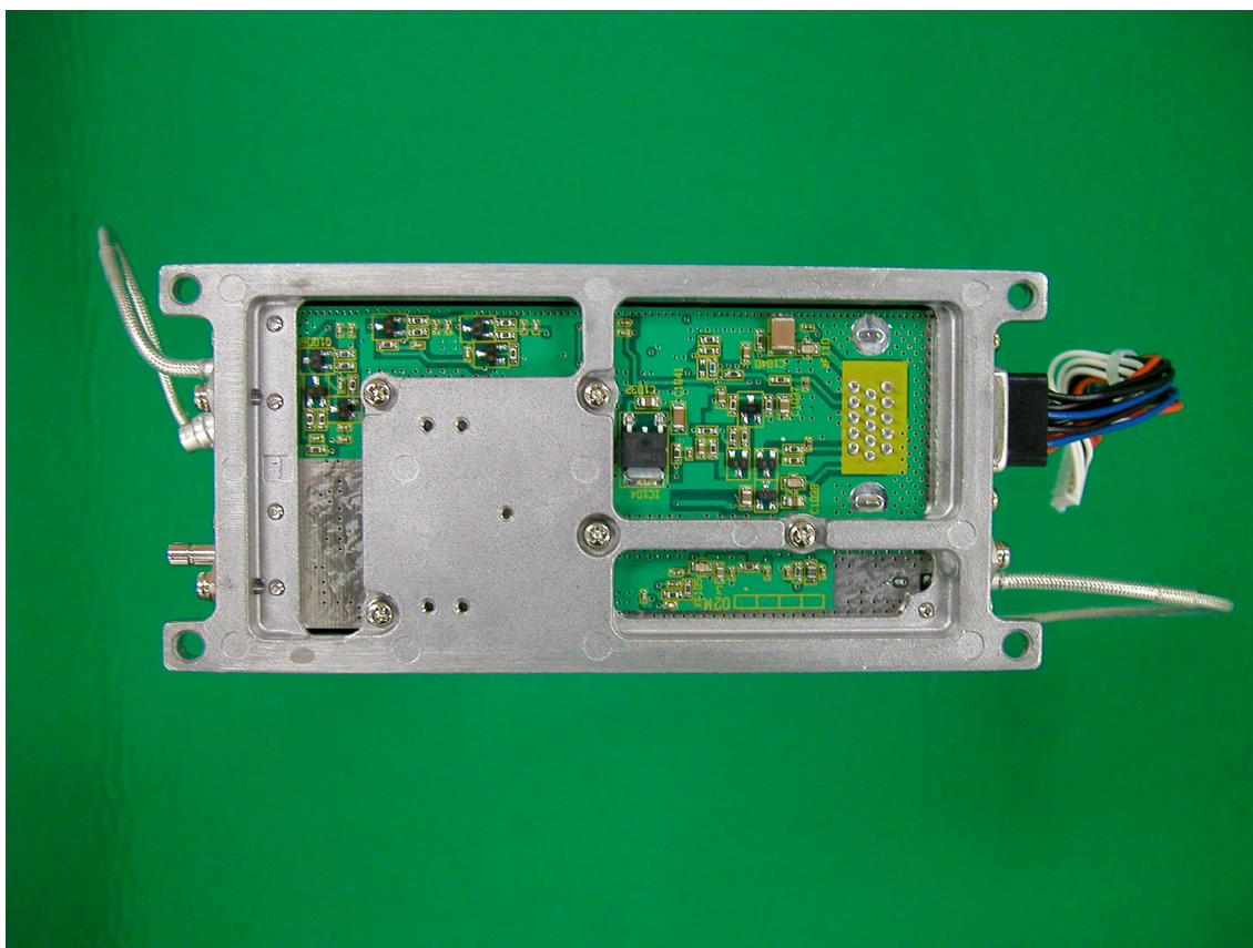
10 Front end module (back)
