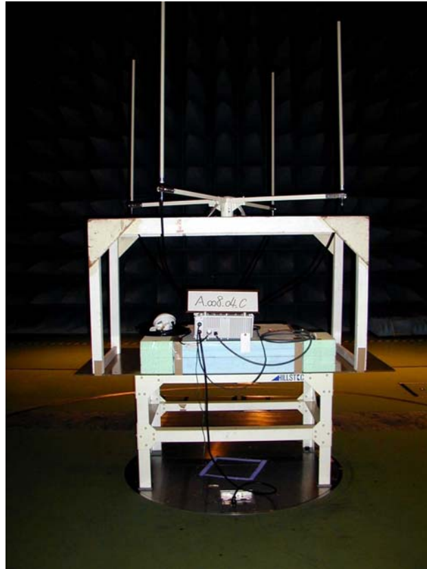
REAR VIEW
