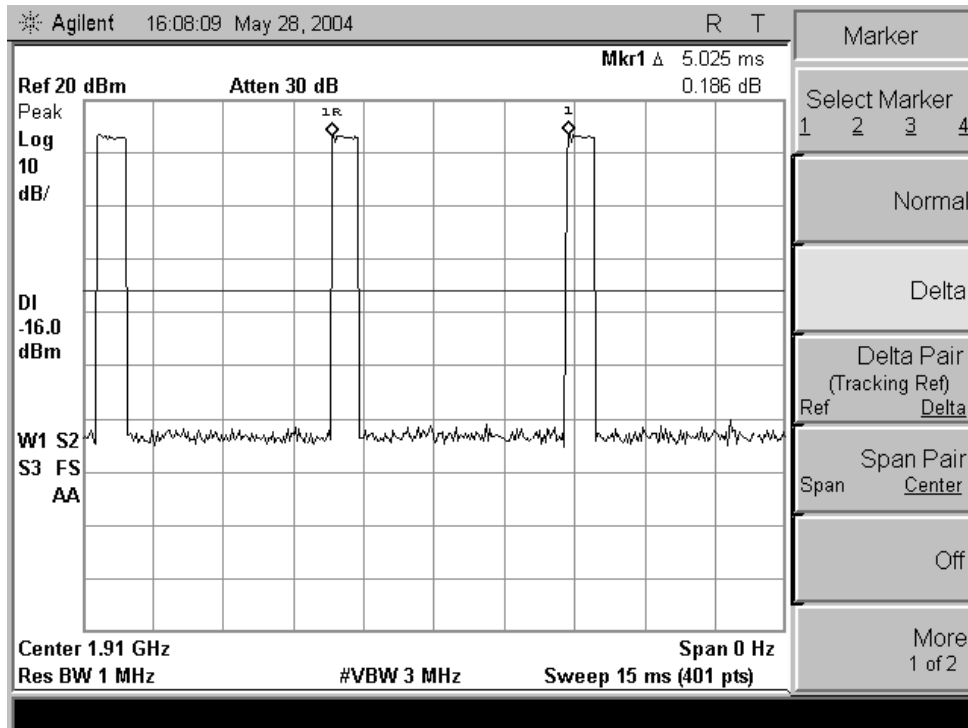
figure 1 (Modulation Characteristics)
