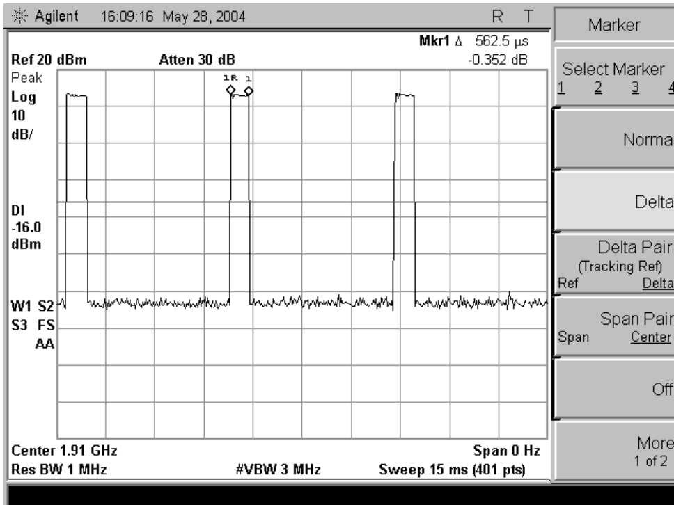
figure 2 (Modulation Characteristics)
