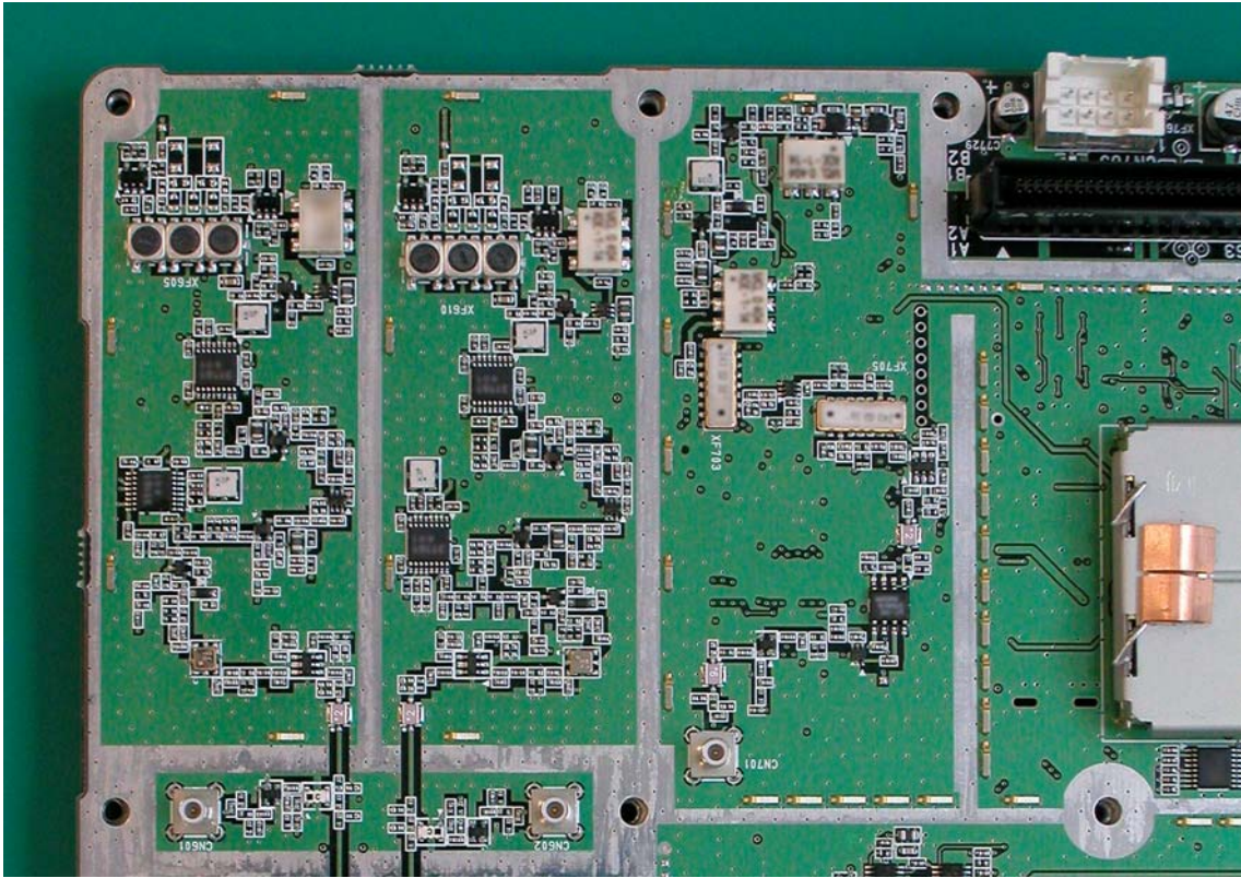
23-1 *RFMB board –front view (Part 1)
