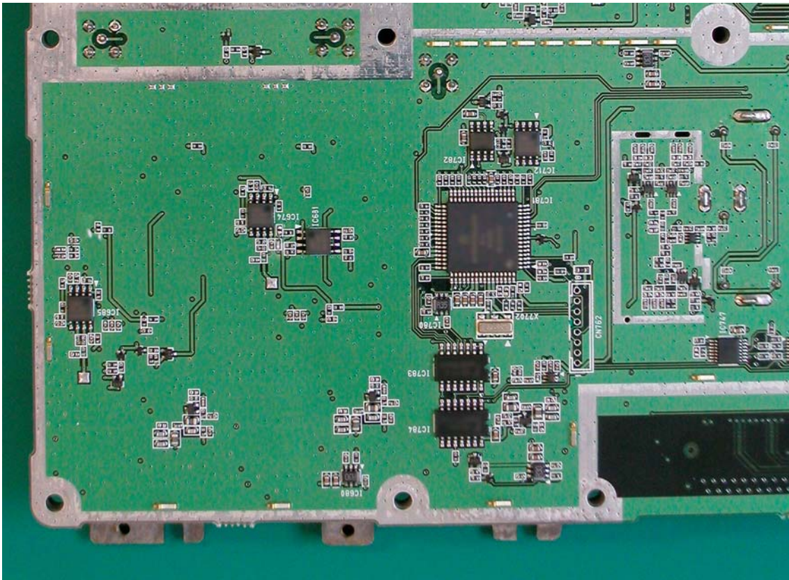
24-2 *RFMB board –back view (Part 2)
