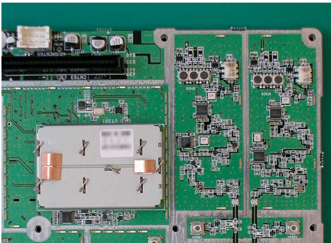
23-3 *RFMB board –front view (Part 3)
