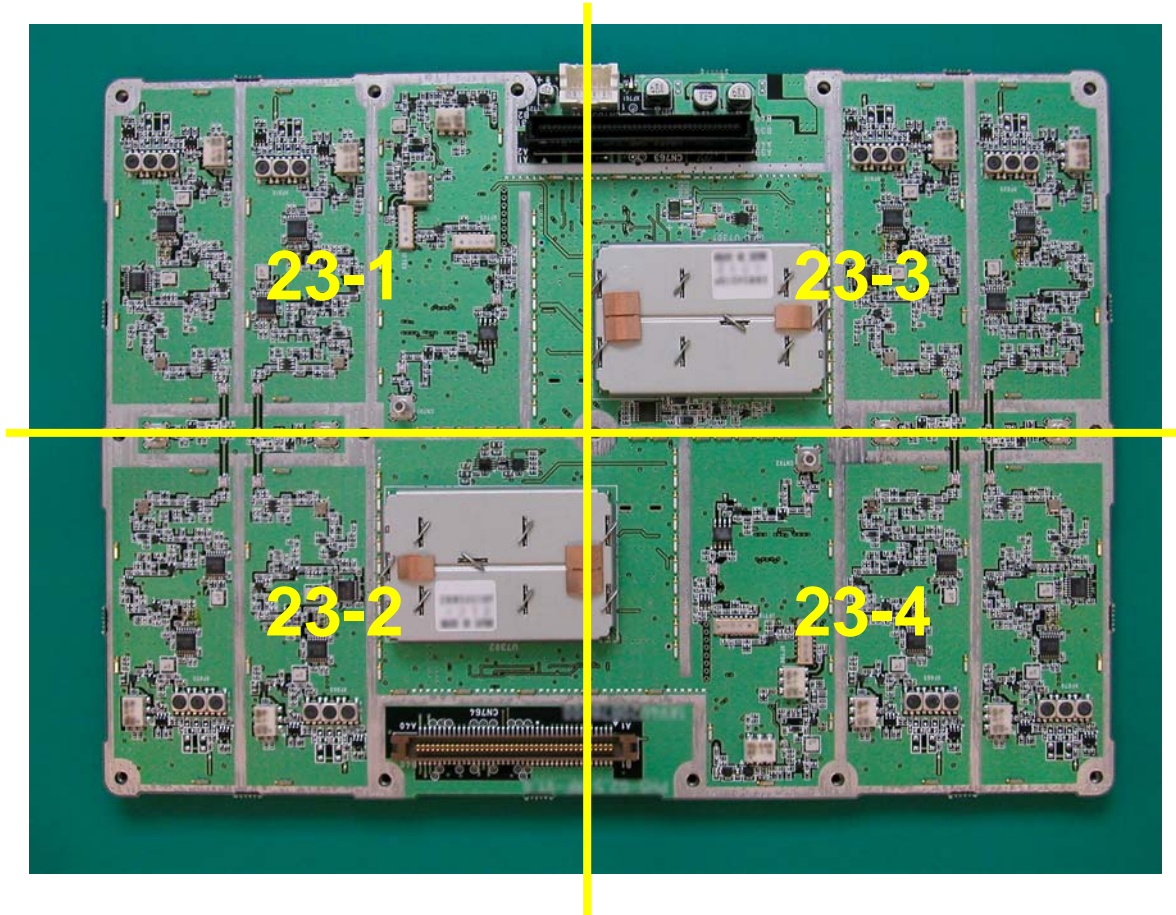
23 RFMB board (front view)
