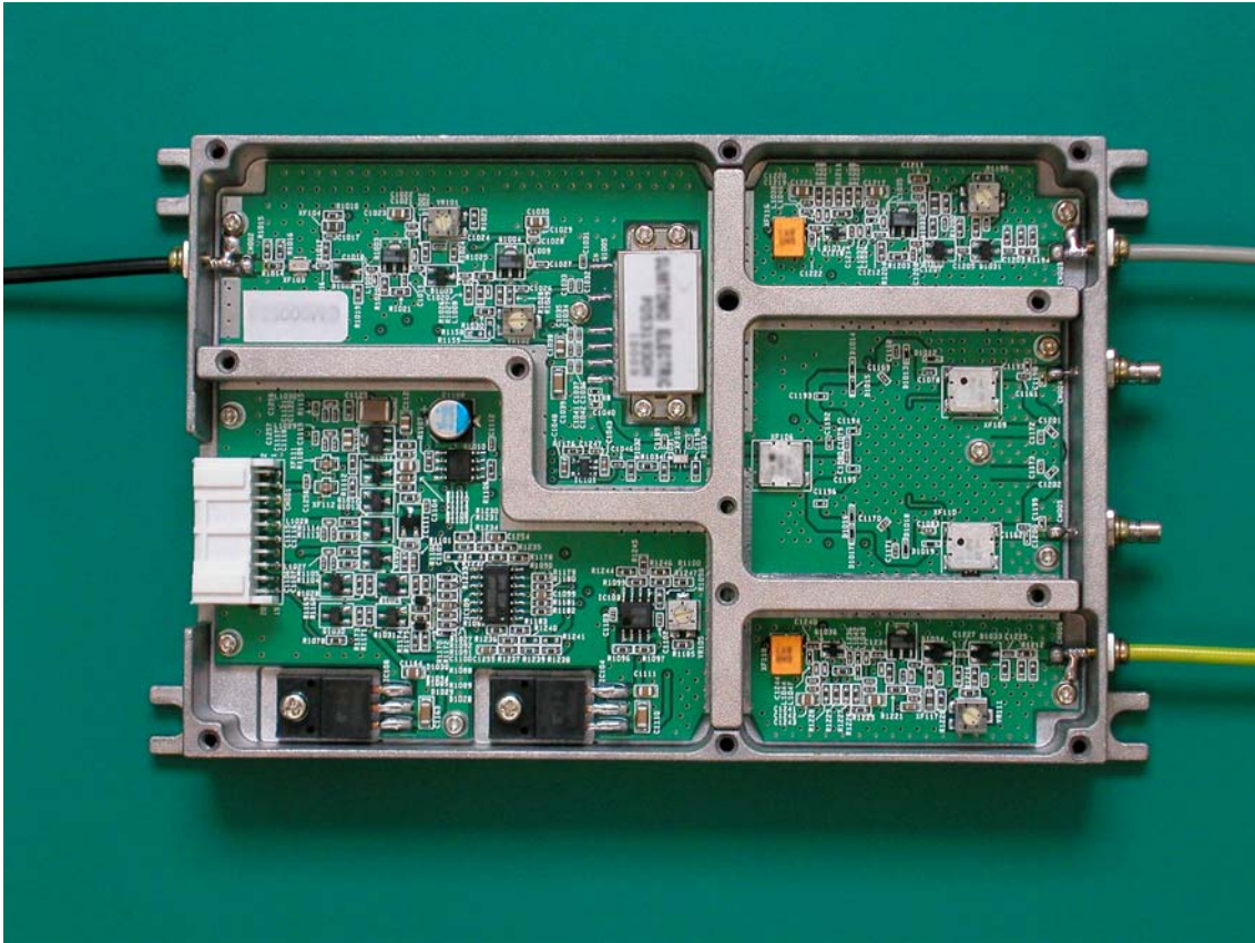
27 Front end module (without cover, front view)
