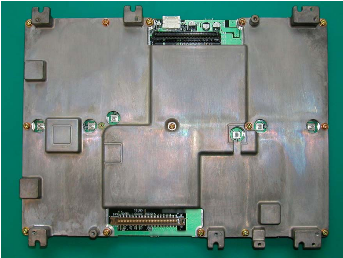
21 RFMB board (with sealed case, front view)
