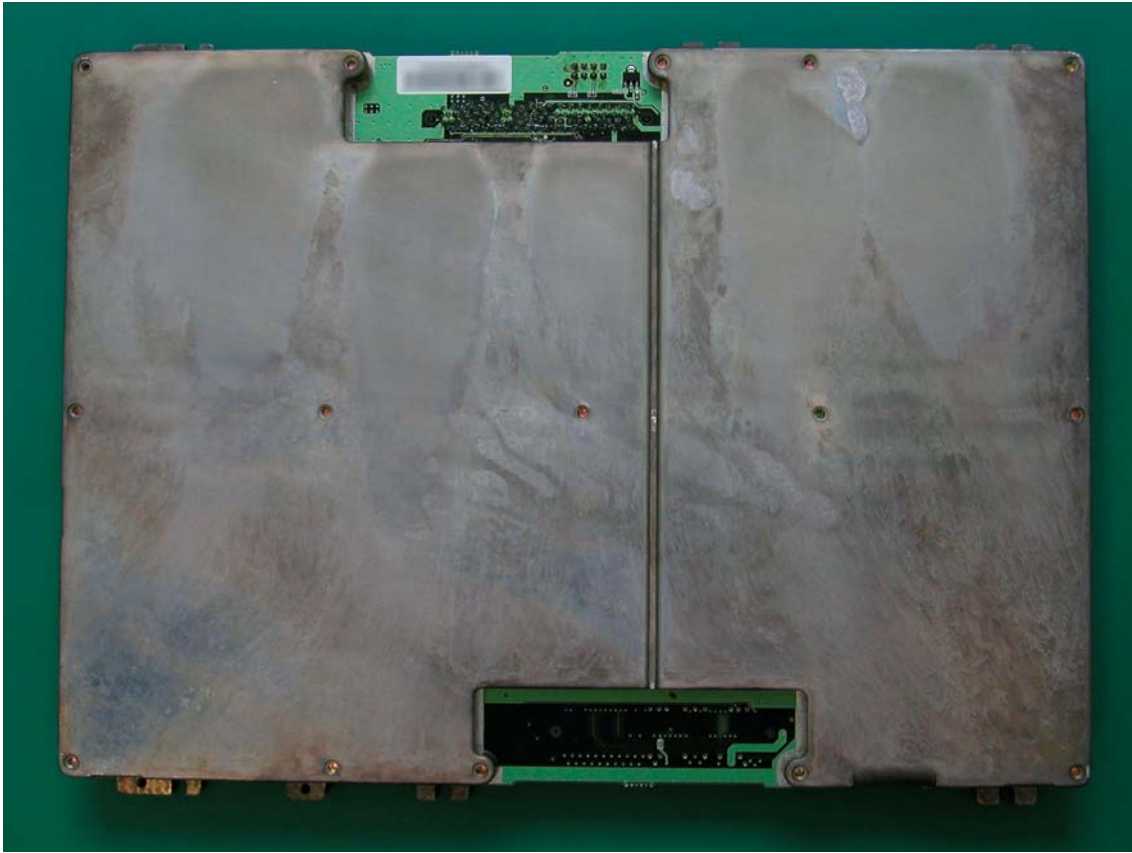
22 RFMB board (with sealed case, back view)
