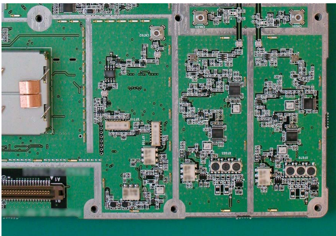
23-4 *RFMB board –front view (Part 4)
