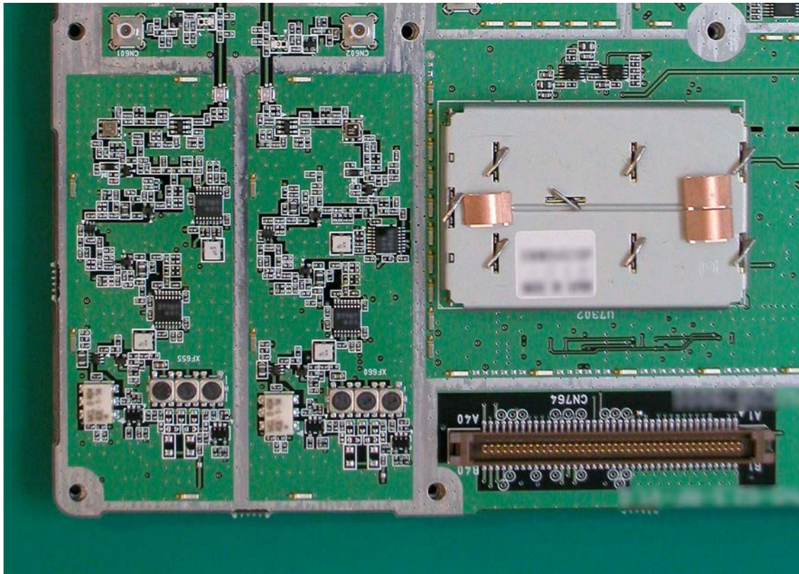
23-2 *RFMB board –front view (Part 2)
