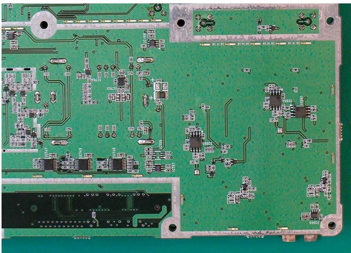
24-4 *RFMB board –back view (Part 4)
