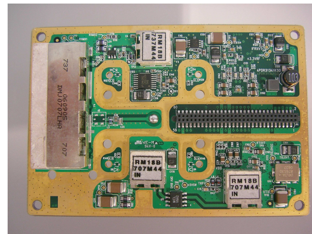
RF Board View (S-side)
