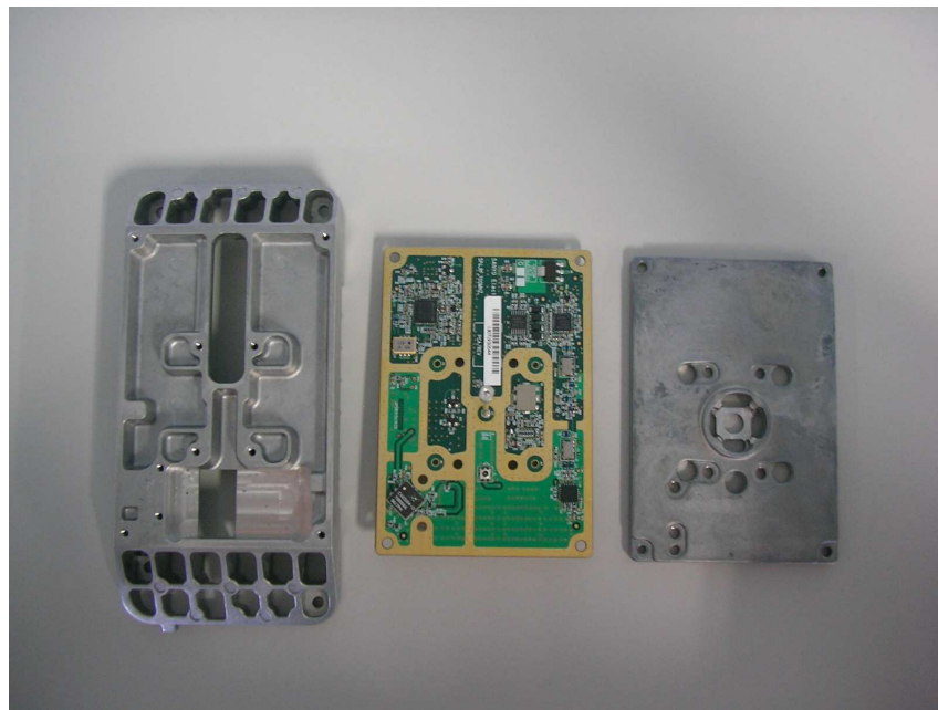
Inside Chassis RF Board Exploded View
