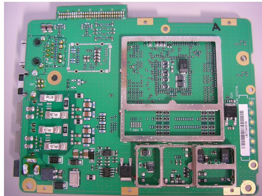
BB Board View (S-side)
