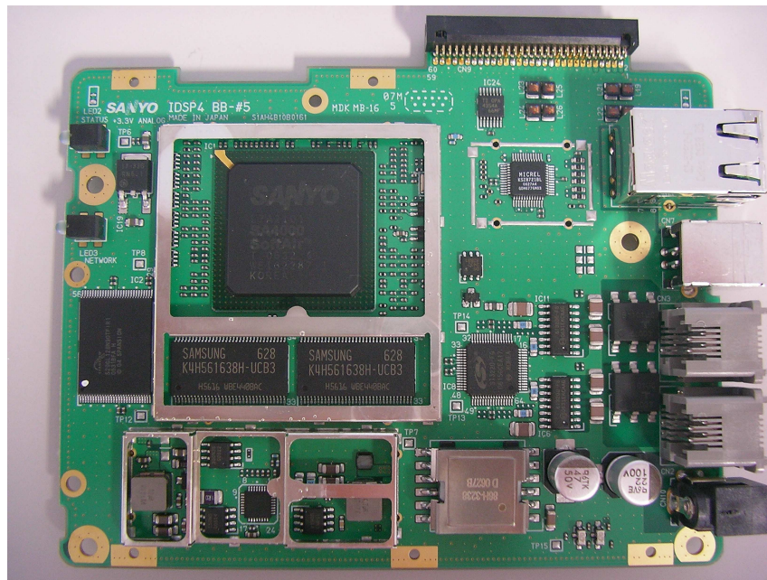
BB Board View (C-side)
