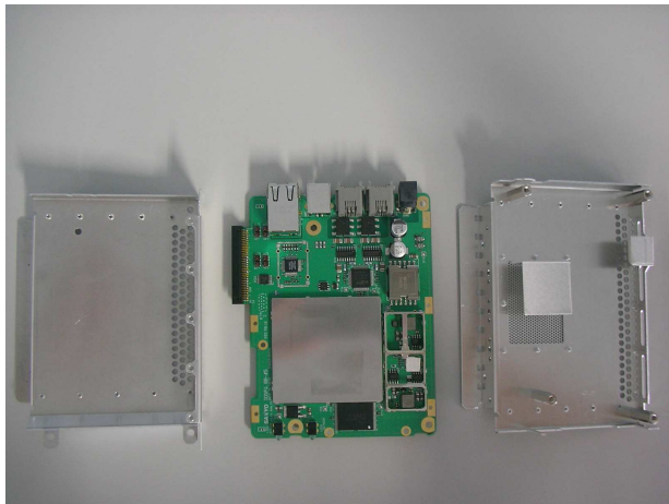
Inside Chassis BB Board Exploded View (1)
