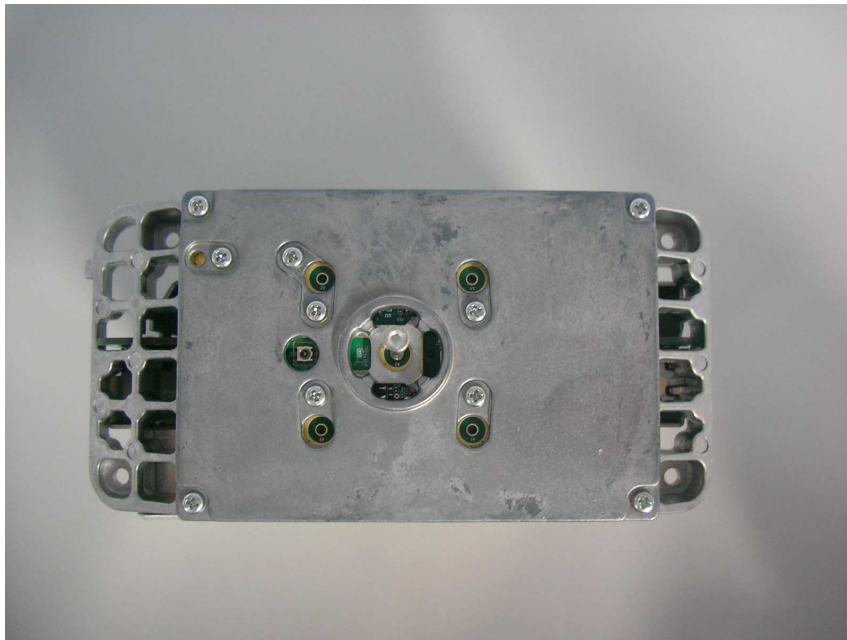
Inside Chassis Top View
