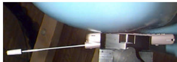
Figure 14. Head SAR Test Setup
