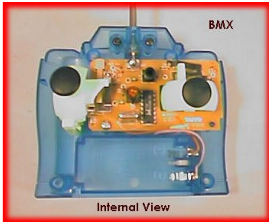
Internal Construction
