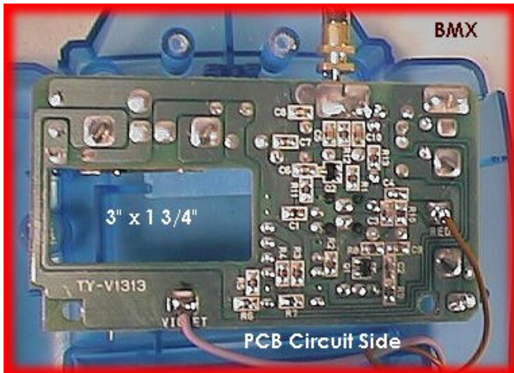
PCB Solder Side
