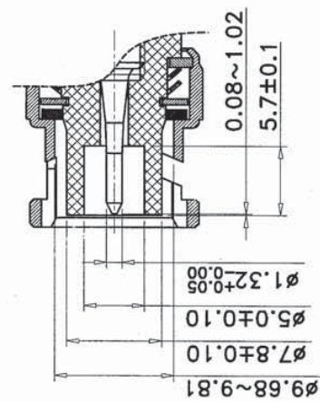
BNC-Plug Connector Interface Mating Dimensions
