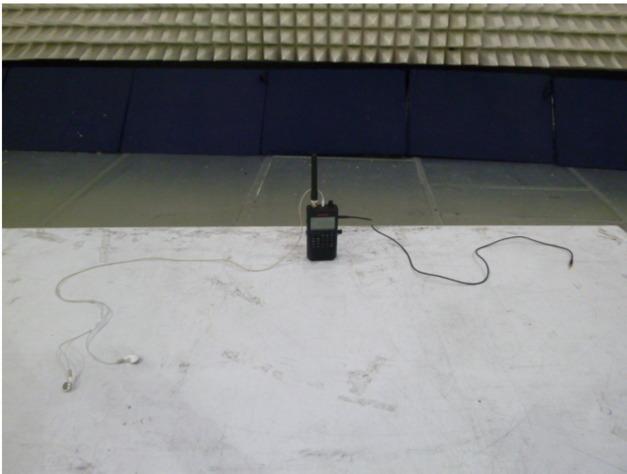
Test Setup Photos FCC ID: ADV0908900 IC: 5088A-PSR120
