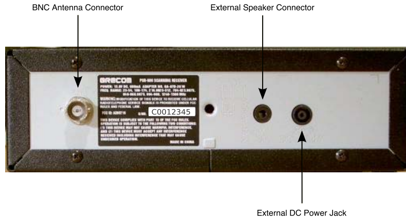
Figure 2 - 0716 rear view
