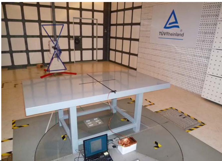
Photograph 2: Set-up for Spurious Emissions (Back View)
