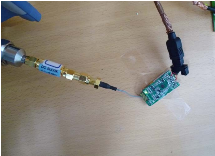
Photograph 4: Set-up for Conducted testing
