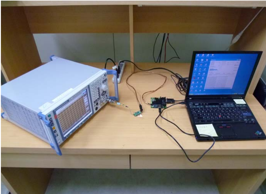
Photograph 3: Set-up for Conducted testing
