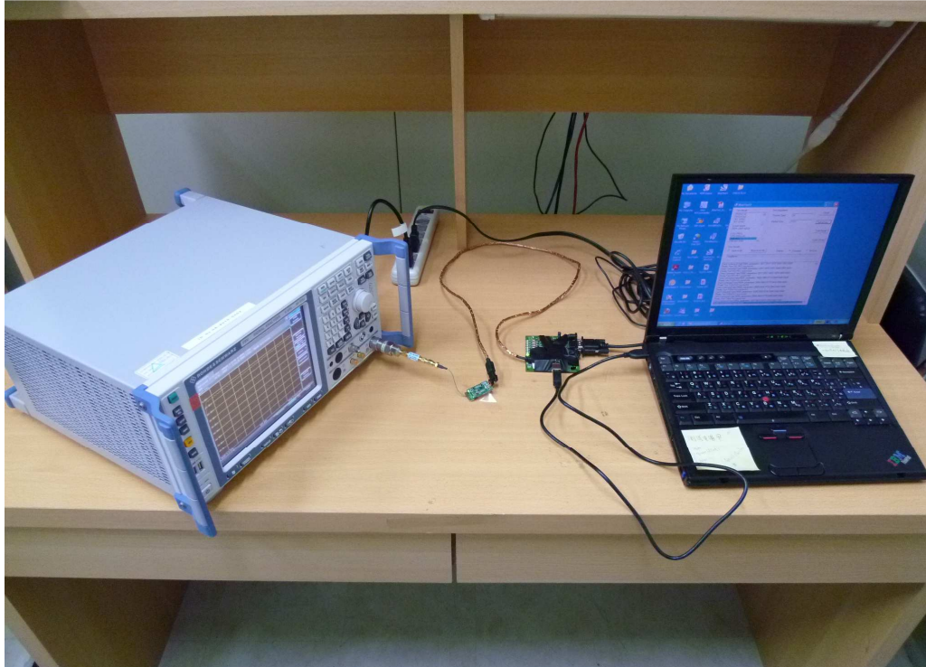
Photograph 3: Set-up for Conducted testing
