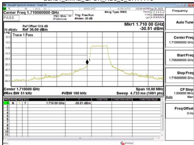
Band4_5MHz_QPSK_RB6_0_CH19975
