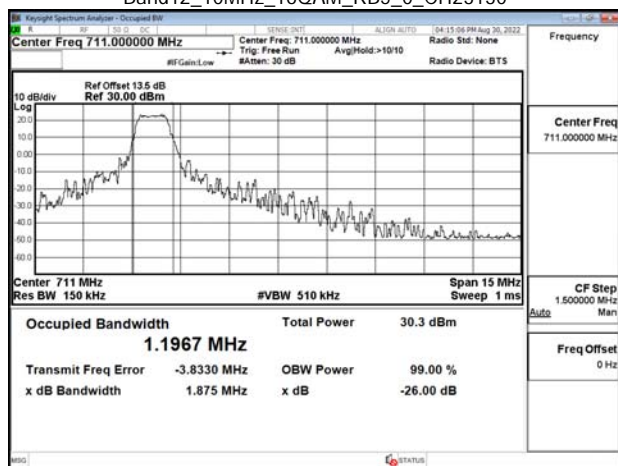
Band12_10MHz_16QAM_RB5_0_CH23130
