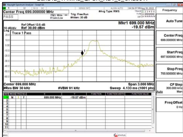
Band12_1.4MHz_QPSK_RB1_0_CH23017
