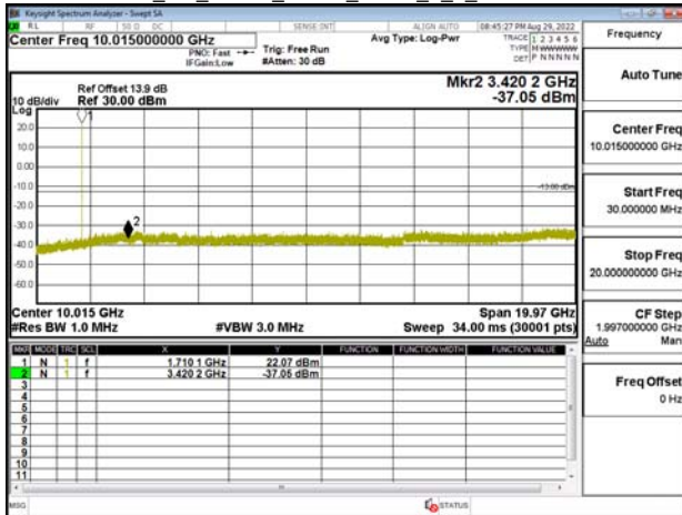
NB_IoT_Band4_15kHz_BPSK_1_0_CH20175
