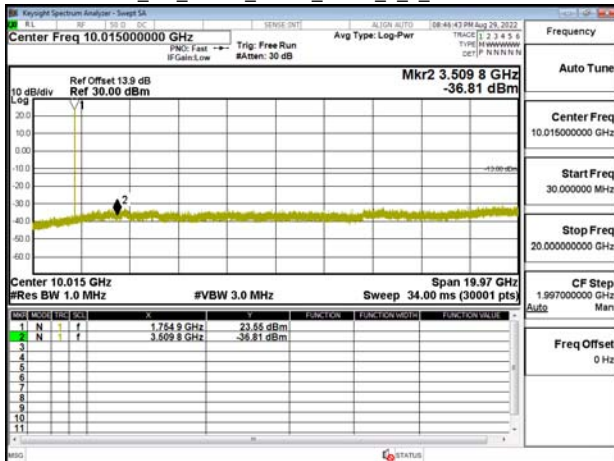
NB_IoT_Band4_15kHz_BPSK_1_0_CH20399
