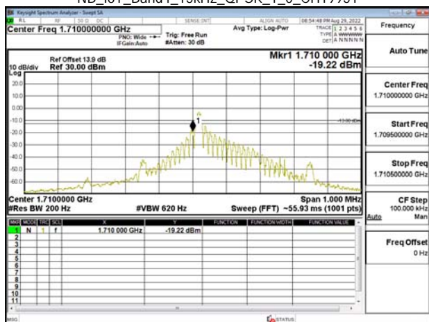
NB_IoT_Band4_15kHz_QPSK_1_0_CH19951
