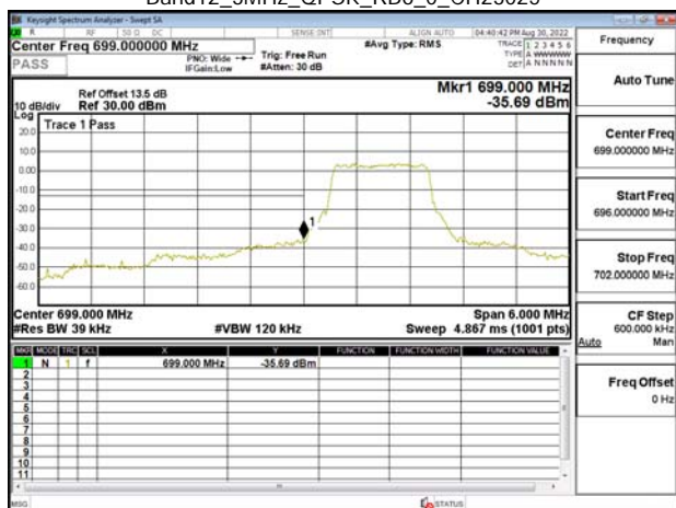
Band12_3MHz_QPSK_RB6_0_CH23025
