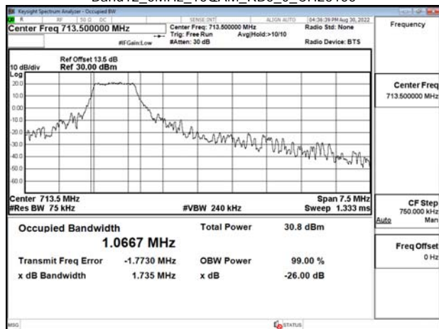
Band12_5MHz_16QAM_RB5_0_CH23155
