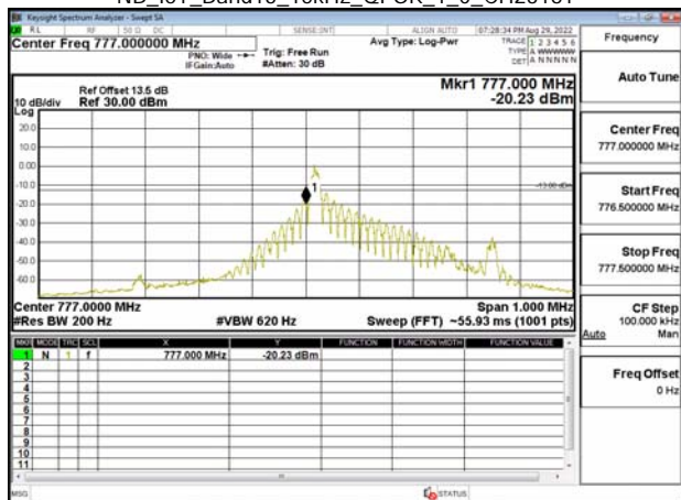
NB_IoT_Band13_15kHz_QPSK_1_0_CH23181
