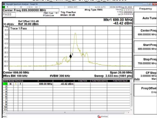
Band12_10MHz_QPSK_RB1_0_CH23060
