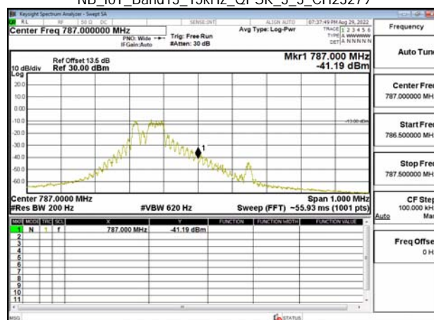
NB_IoT_Band13_15kHz_QPSK_3_3_CH23279
