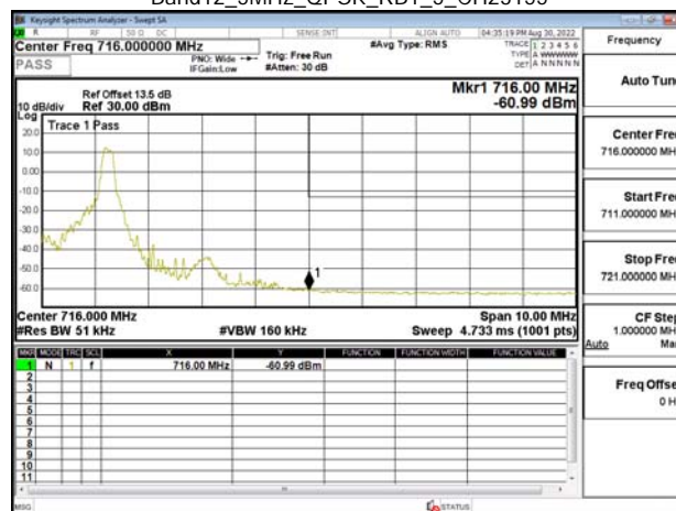
Band12_5MHz_QPSK_RB1_5_CH23155
