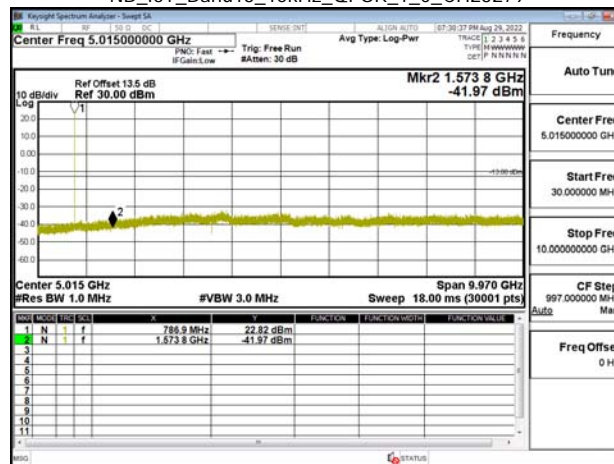
NB_IoT_Band13_15kHz_QPSK_1_0_CH23279
