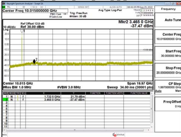
NB_IoT_Band4_15kHz_BPSK_1_0_CH20399
