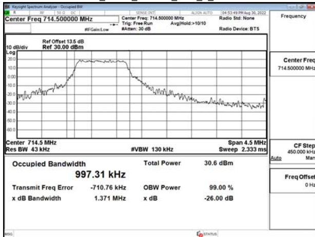
Band12_3MHz_16QAM_RB5_0_CH23165
