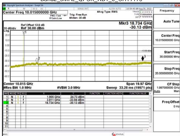
Band2_5MHz_QPSK_RB1_0_CH19175
