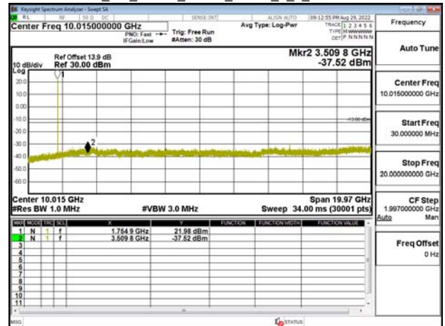
NB_IoT_Band4_15kHz_QPSK_1_0_CH20399
