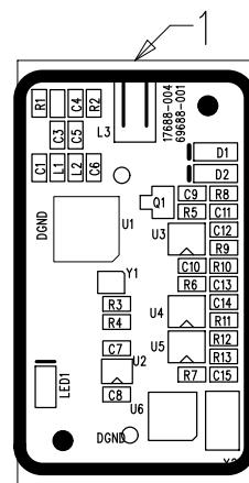
SILKSCREEN TOP
