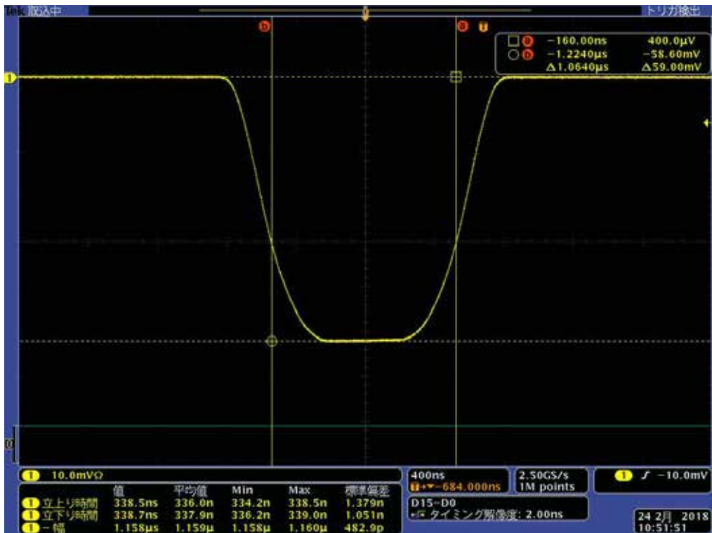
Fig. 6.22 Long pulse envelope
