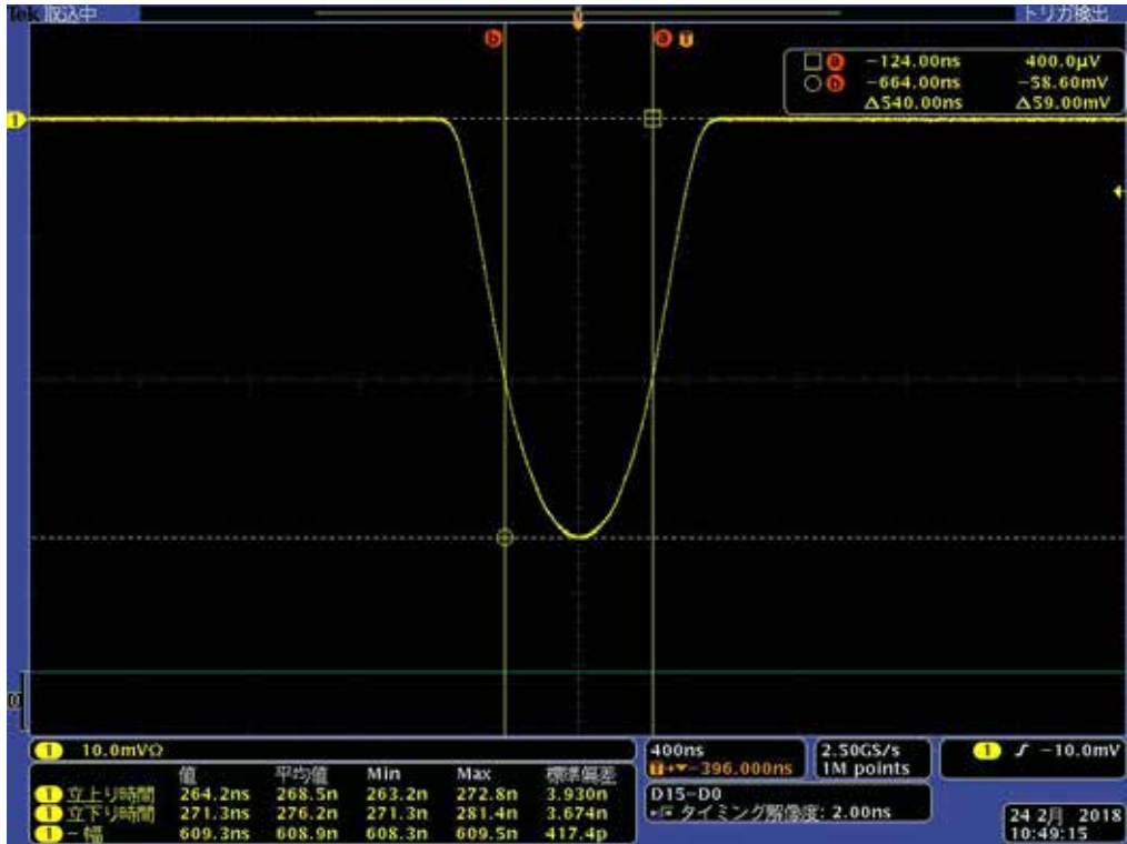
Fig. 6.21 Short pulse envelope
