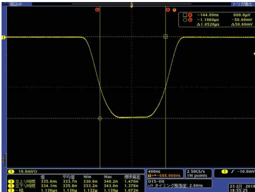
Fig. 6.2 Long pulse envelope
