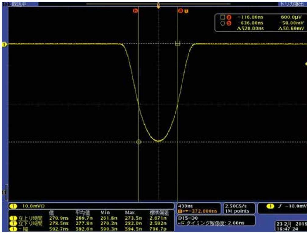
Fig. 6.1 Short pulse envelope
