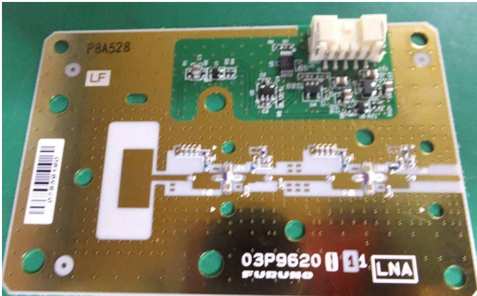
Internal view of 03P9620 front side (LNA)
