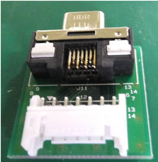
Internal view of 84P0017 (HDR-PHD14)
