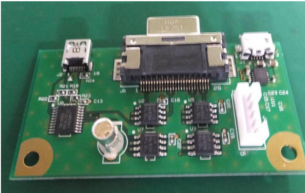
Internal view of 84P0015 (LVCONV)
