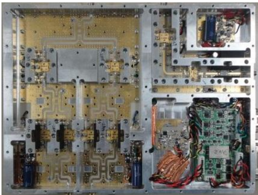
Internal view of the RFCONV:
