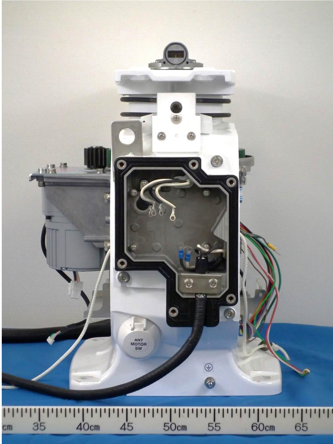
1.1.15 Left side of RSB-146 (with TEMP-SW board 03P9578 removed)
