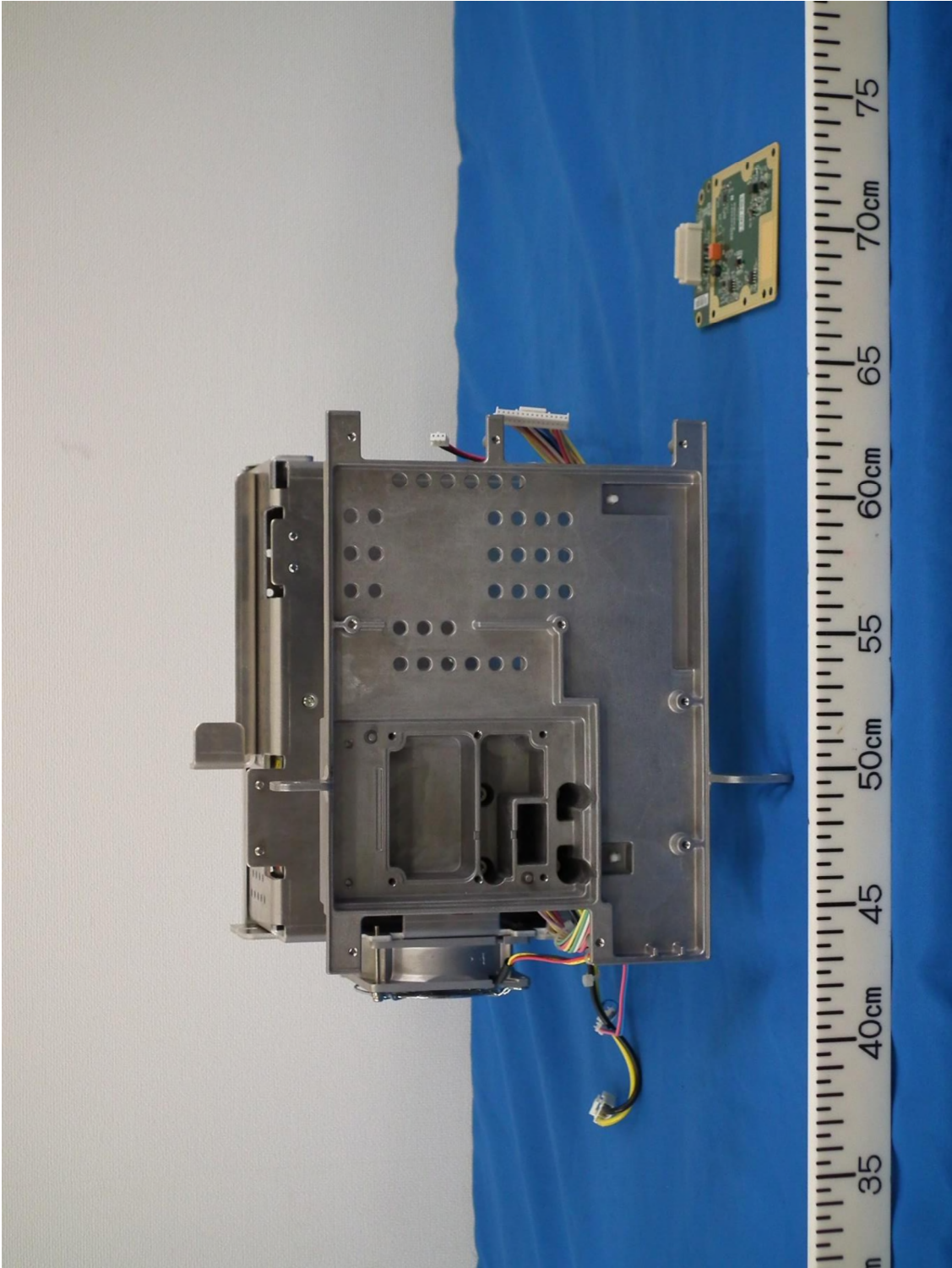
1.2.12 Left view of RTR-132 (with MIC board 03P9567 removed)
