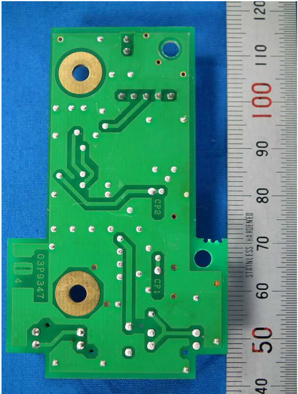
1.26 BP-GEN board 03P9347, Rear side
