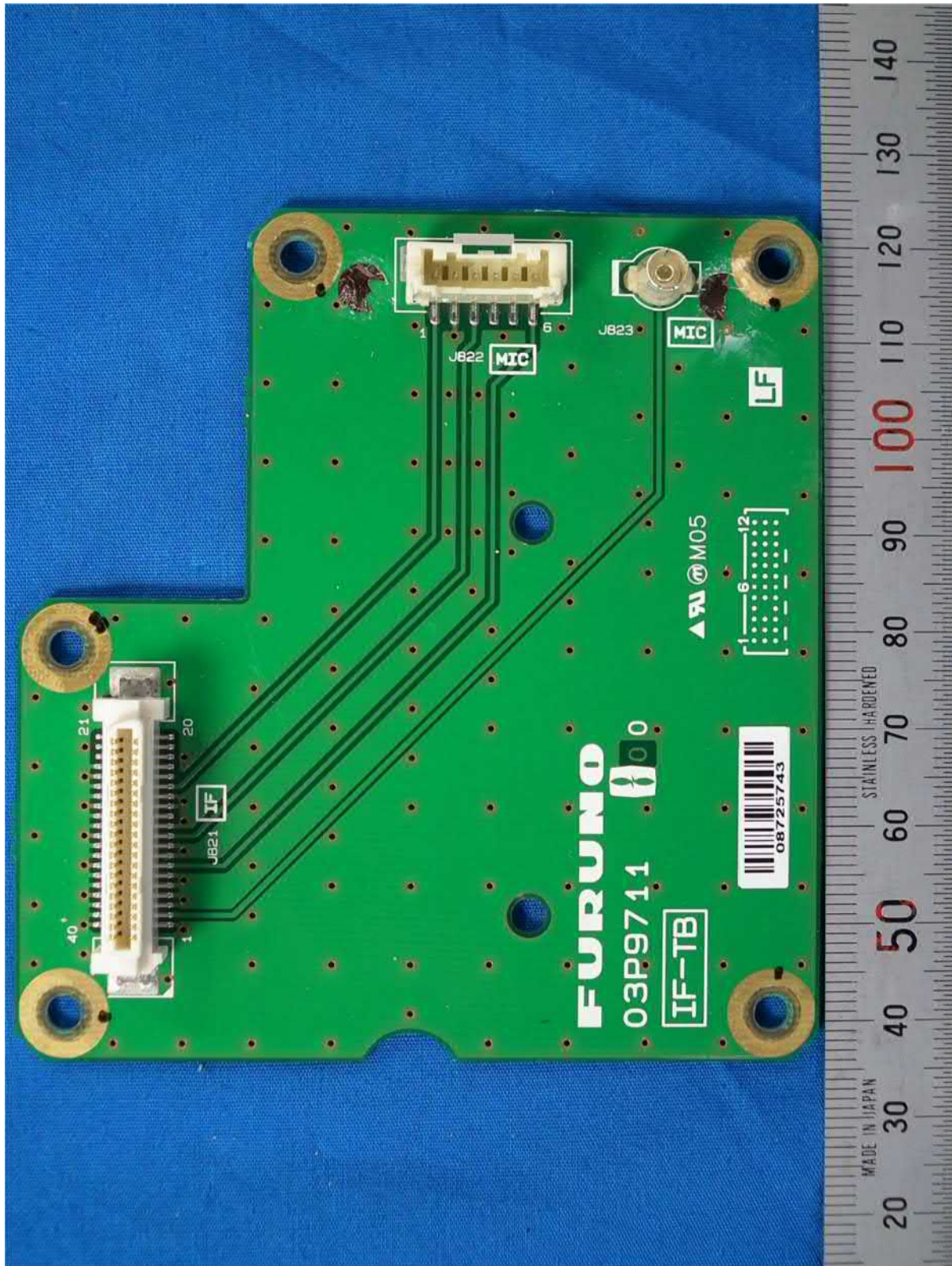
1.15 IF-TB board 03P9711, Front side
