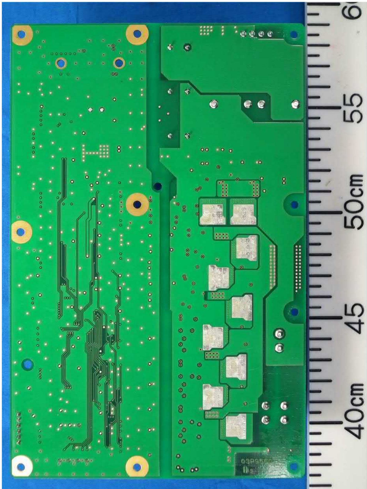
1.22 MTR-DRV board 03P9560, Rear side
