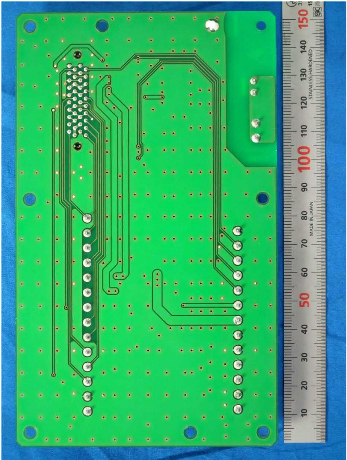
1.24 RF-TB board 03P9712, Rear side
