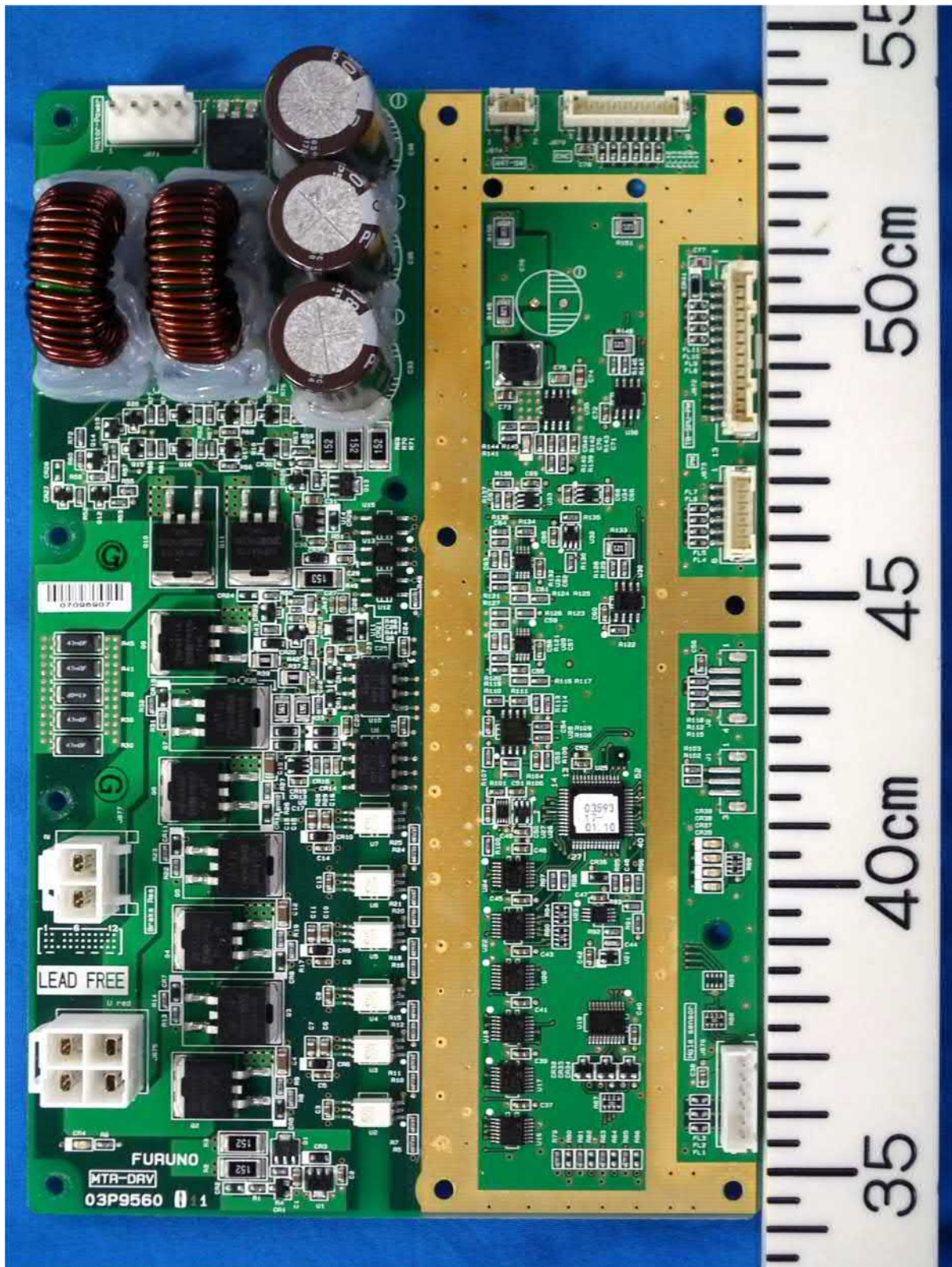
1.21 MTR-DRV board 03P9560, Front side
