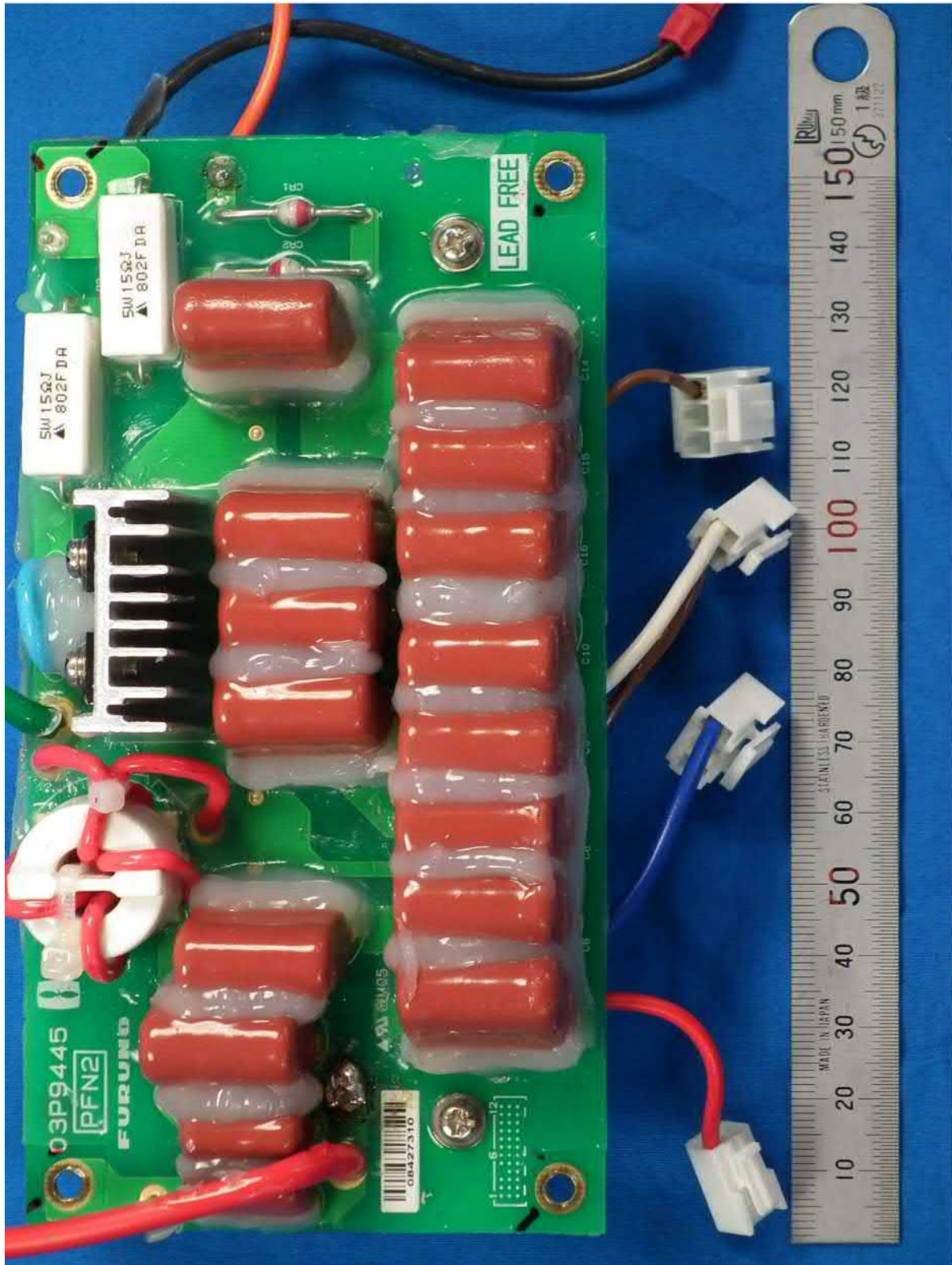
1.7 PFN2 board 03P9445, Front side
