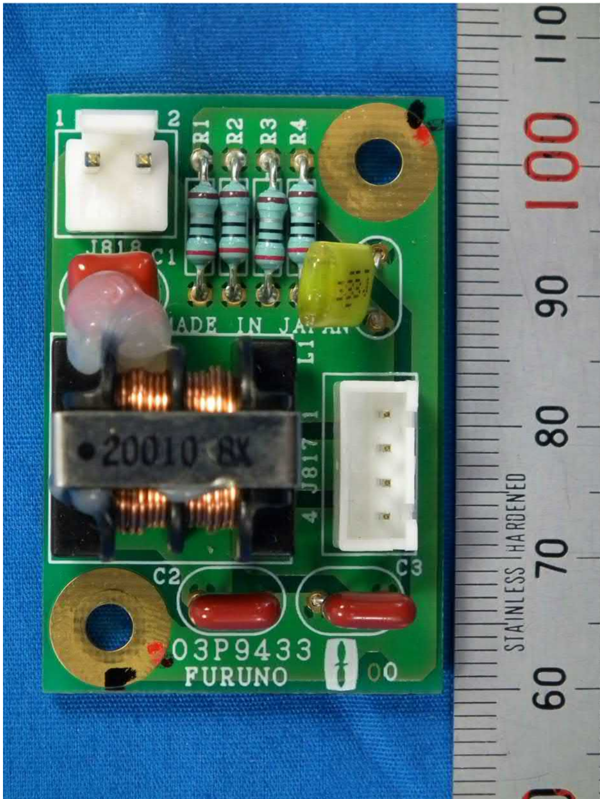
1.9 PFN3 board 03P9433, Front side
