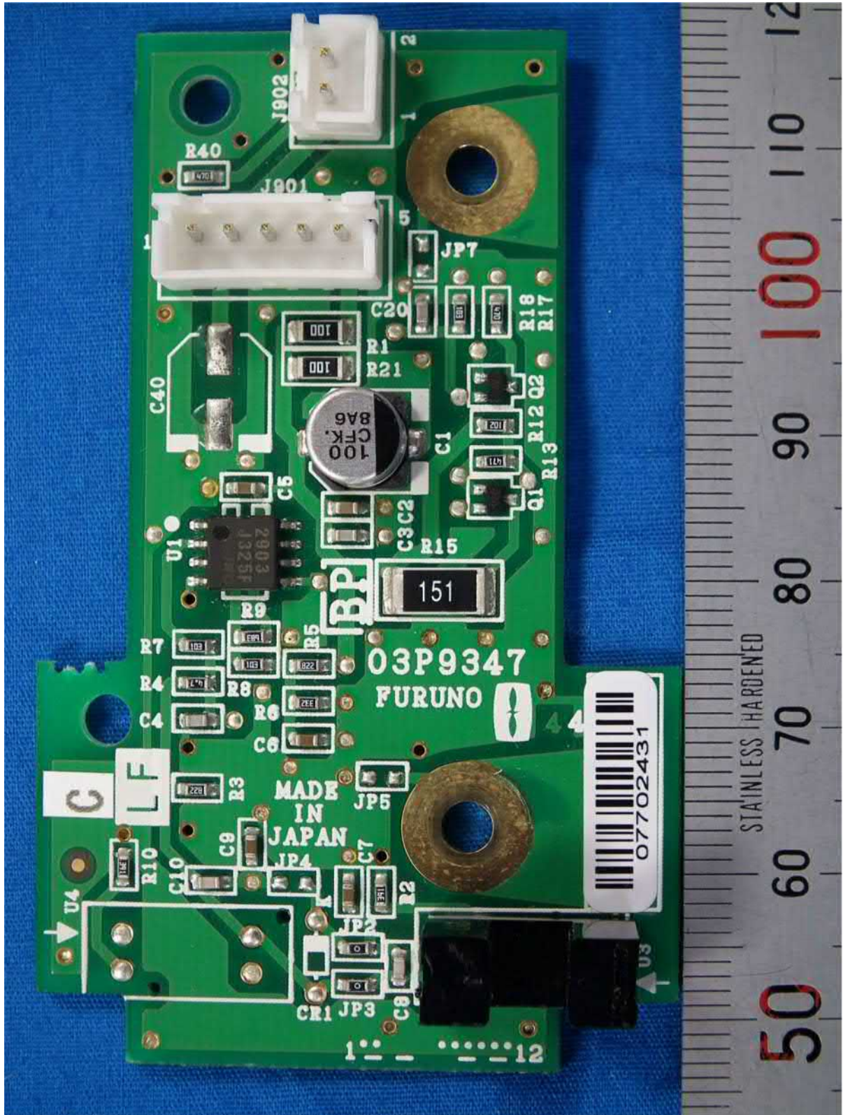
1.25 BP-GEN board 03P9347, Front side
