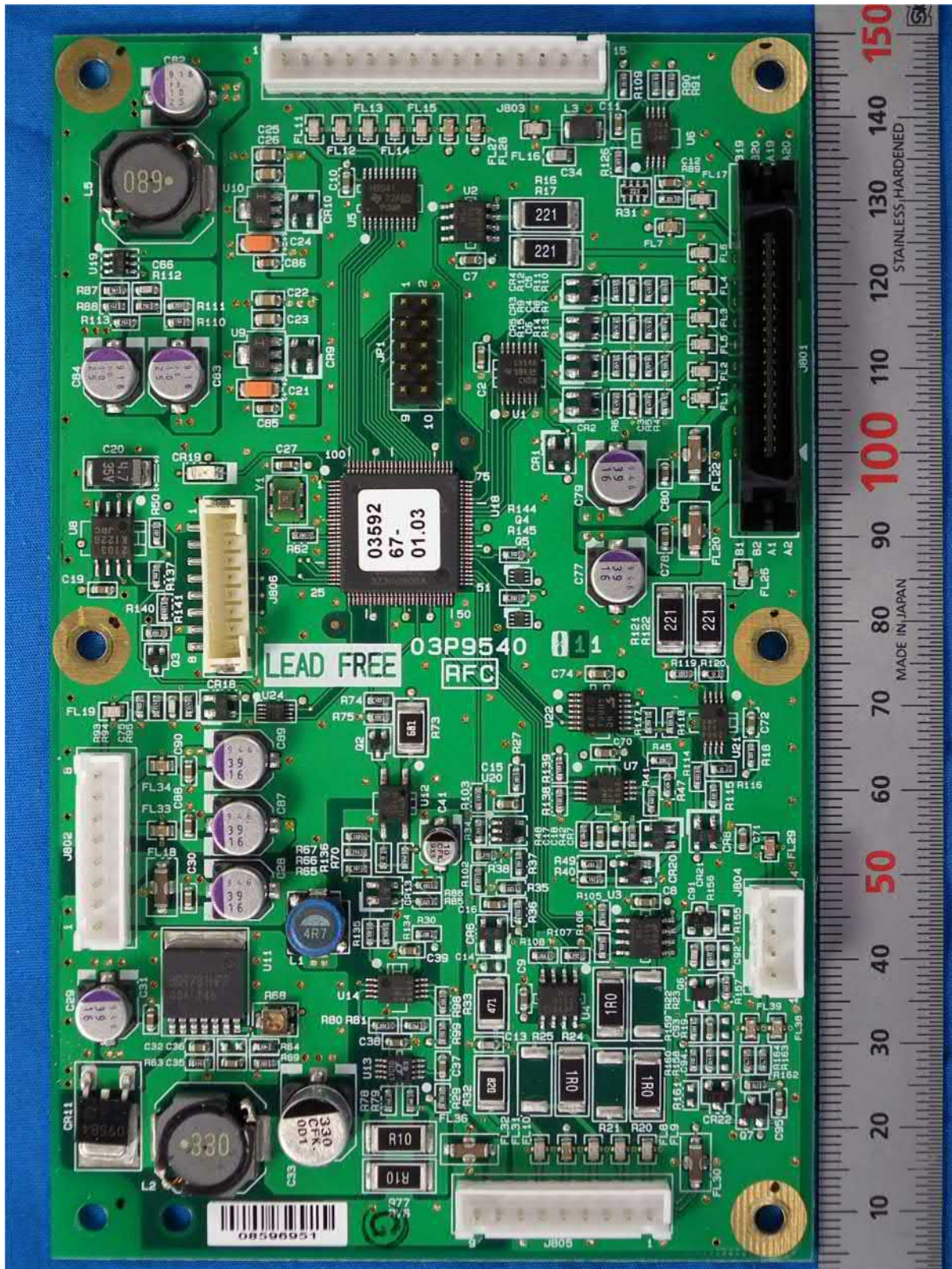
1.19 RFC board 03P9540, Front side
