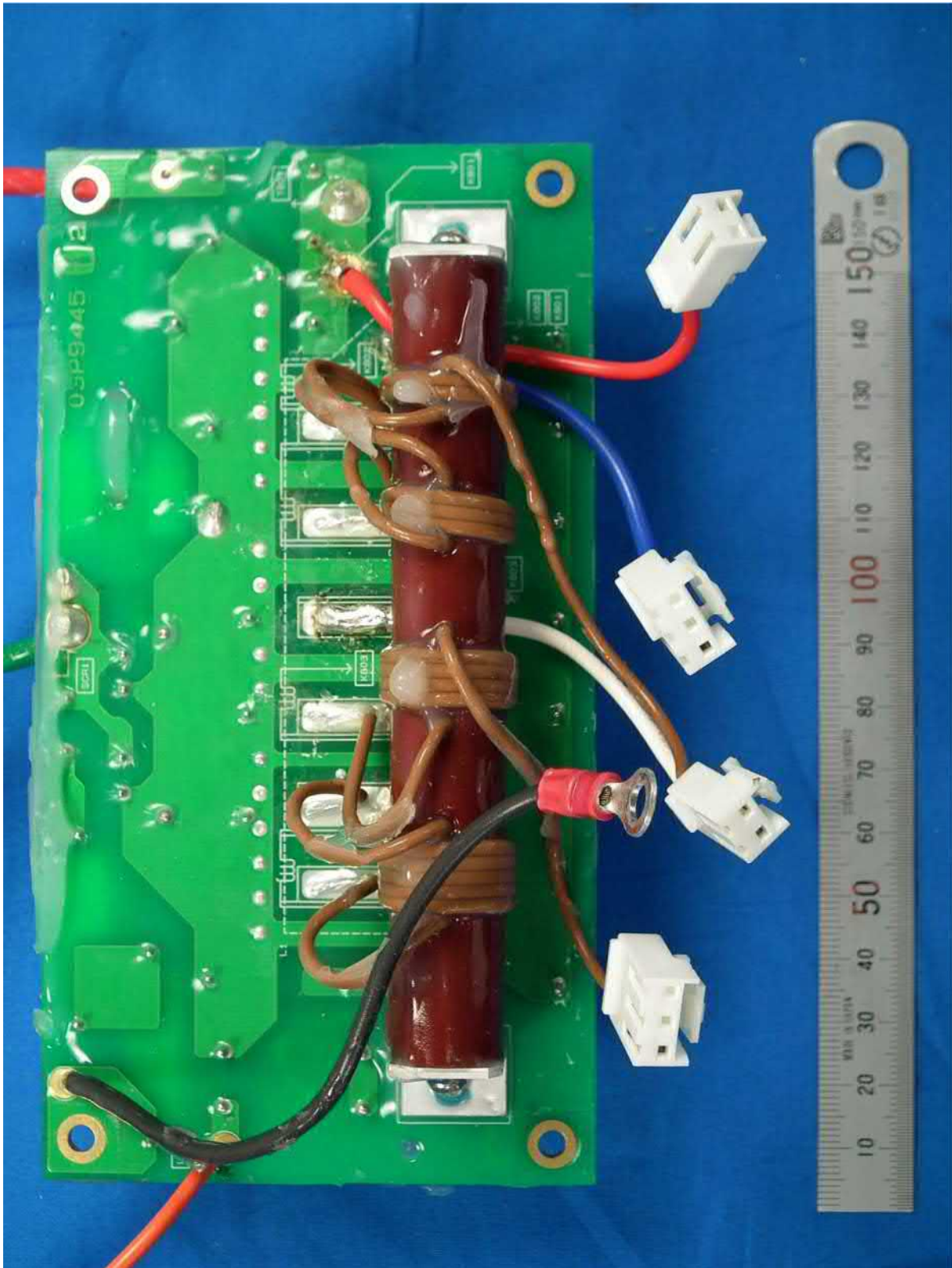
1.8 PFN2 board 03P9445, Rear side
