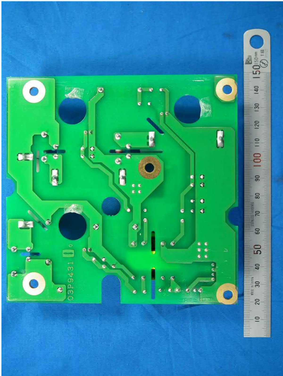
1.6 PFN1 board 03P9431, Rear side
