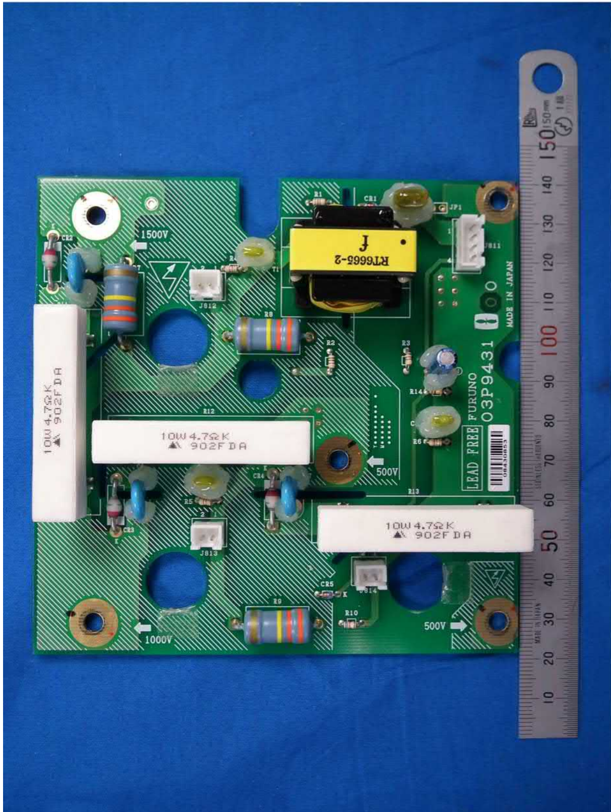
1.5 PFN1 board 03P9431, Front side
