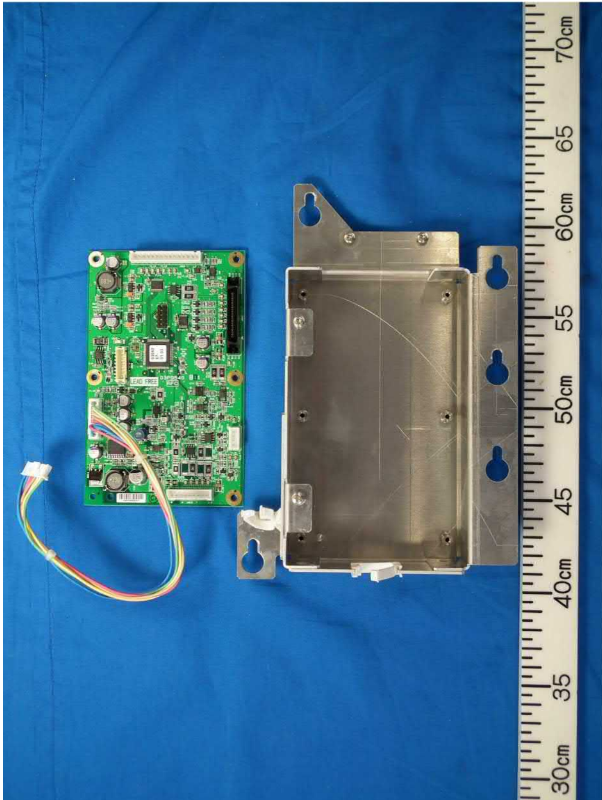
1.8 RFC board module (with removed from the metal base part)
