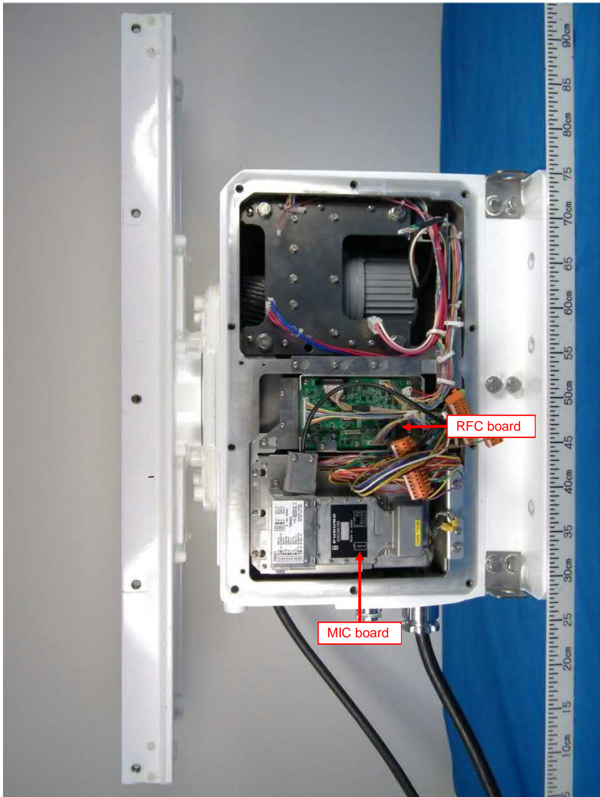
1.6 Right side view (with MTR-DRV board 03P9560 and RF-TB board 03P9712 removed, showing RFC board 03P9540 and MIC board 03P9569)
