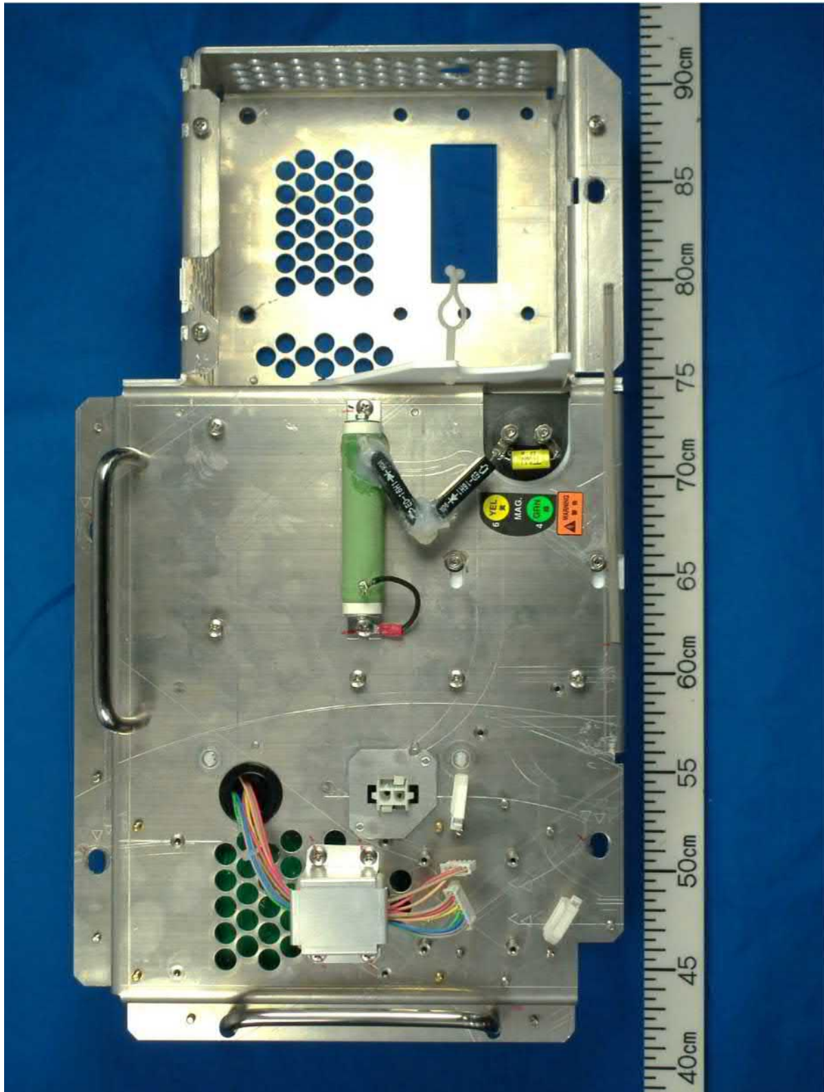
1.20 Transceiver RTR-129, Front side (with BUF board 03P9446 removed)
