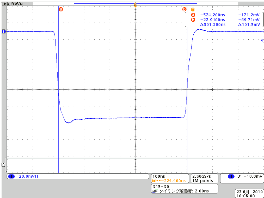
Fig. 6.5 ch1, P0N, M2 pulse envelope
