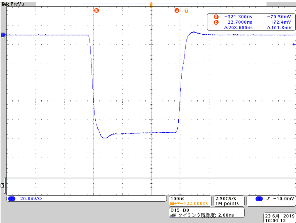
Fig. 6.4 ch1, P0N, M1 pulse envelope
