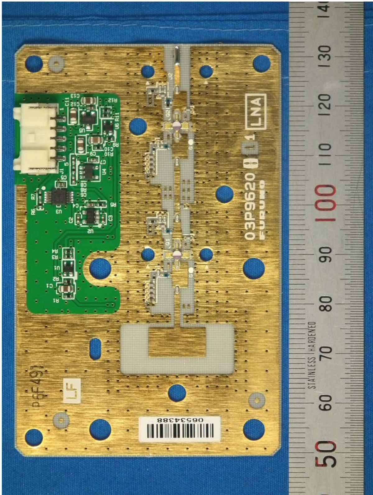
1.2.5 LNA board 03P9620, Front side
