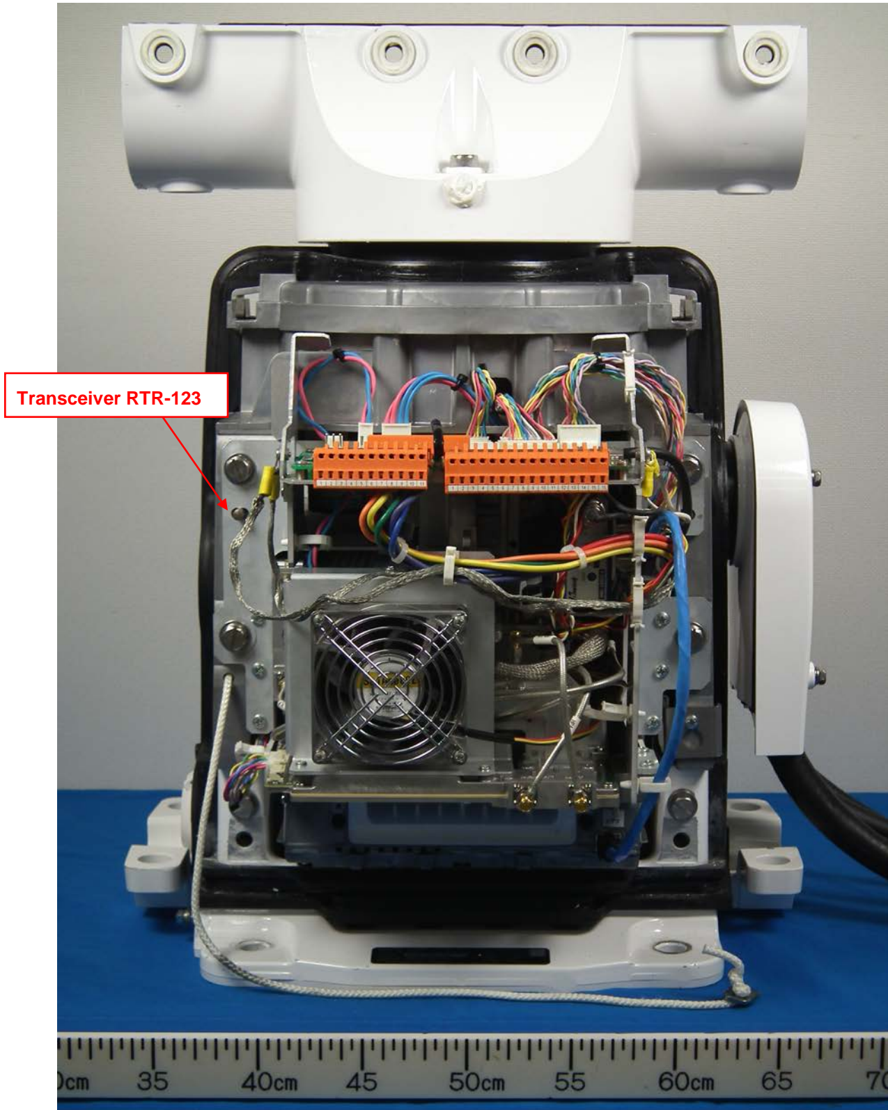
1.1.3 Rear view of RSB-128 (with the rear cover removed, showing Transceiver RTR-123)
