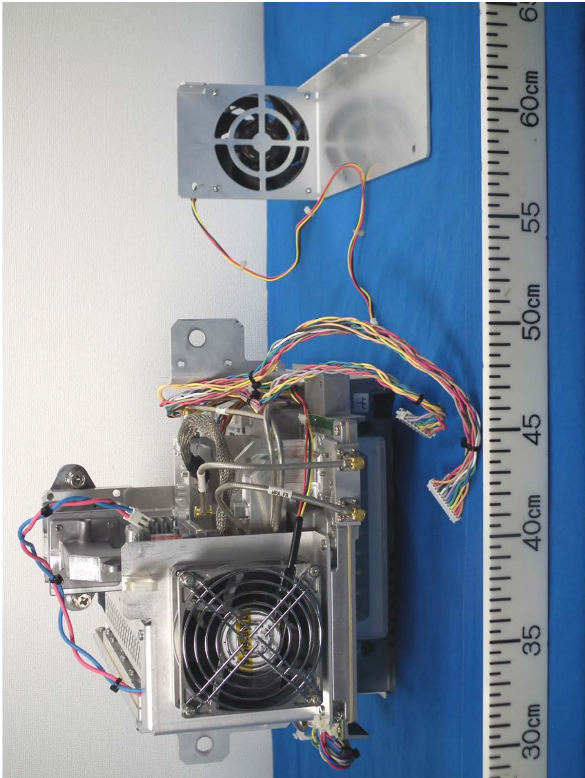
1.2.11 Front view of RTR-123 (with FAN removed)
