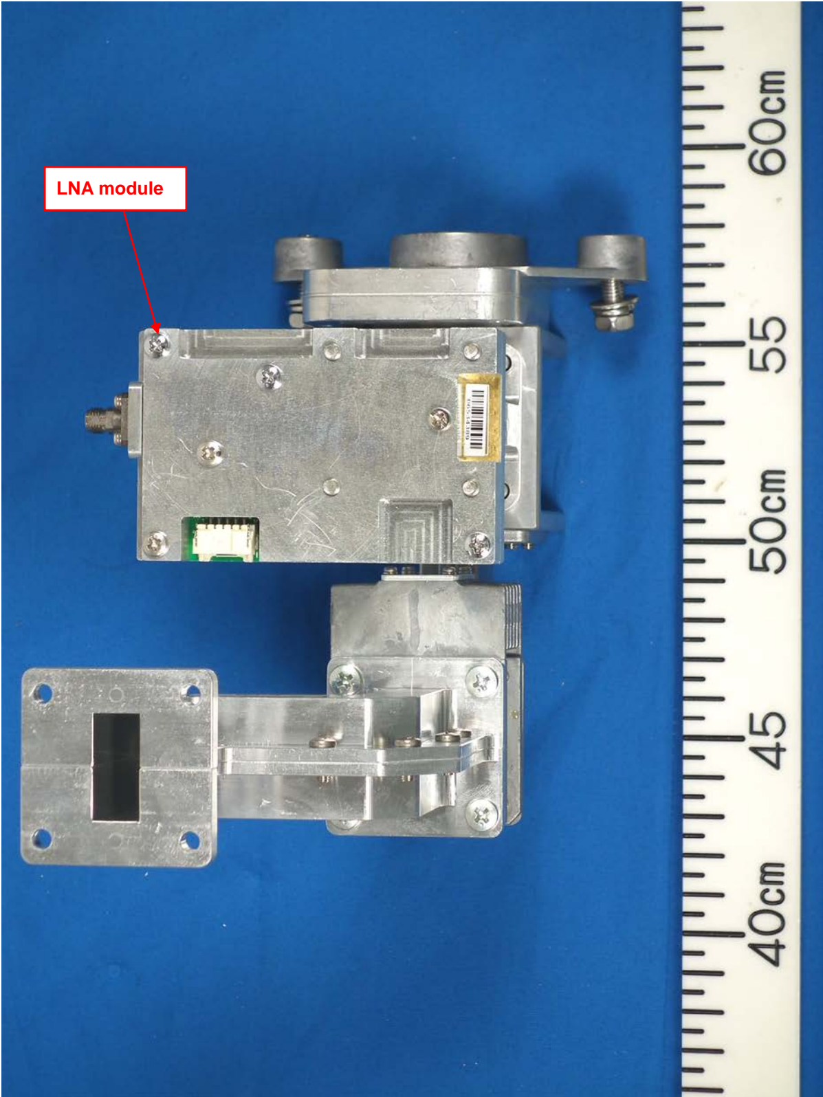
1.2.14 Bottom view of the circulator and limiter module (with LNA module fixed)
