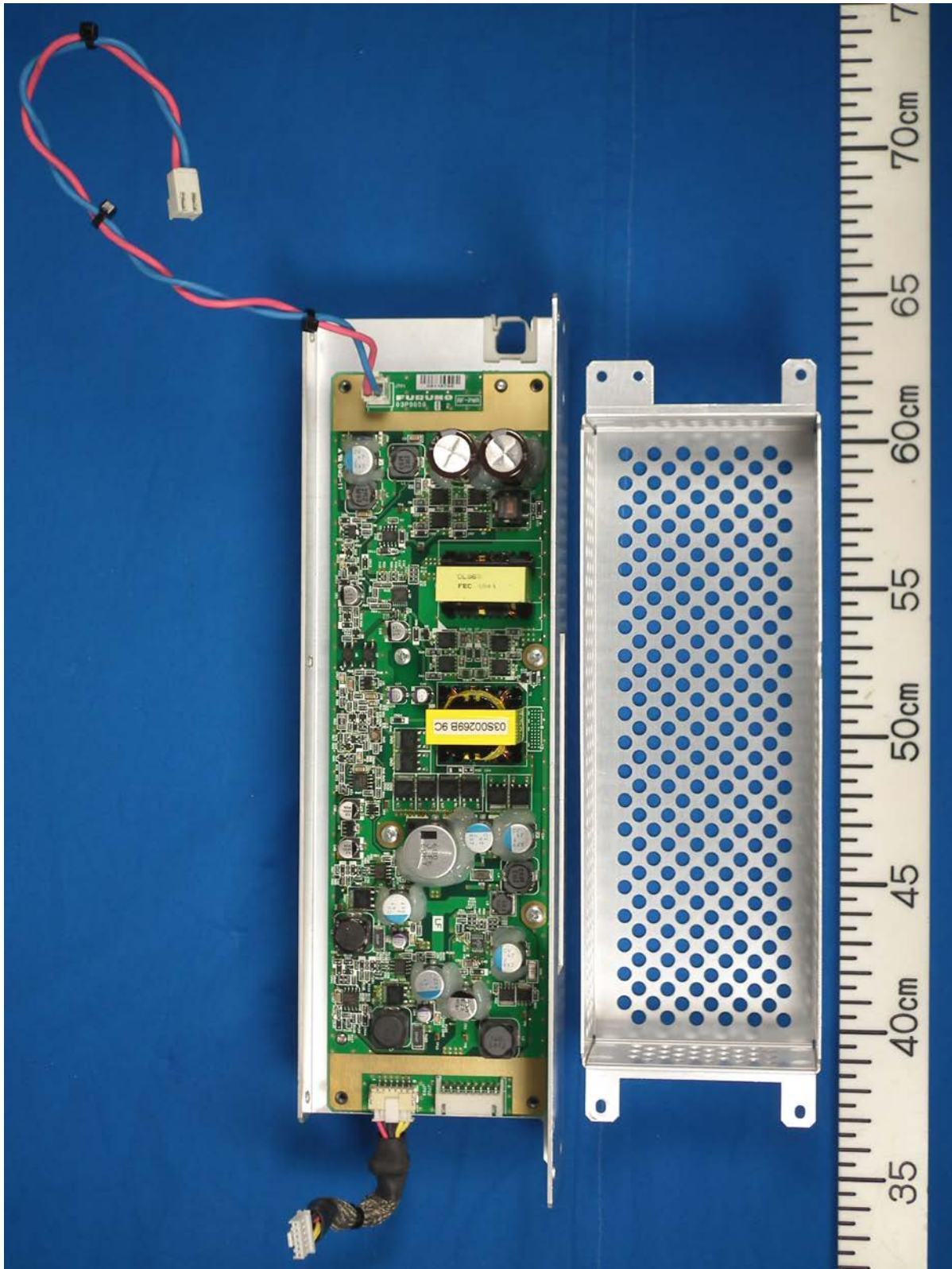
1.2.17 RF-PWR module (with the shielding cover removed, showing RF-PWR board 03P9656)
