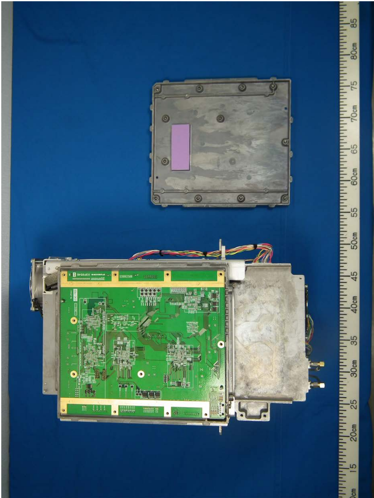
1.2.9 Bottom view of RTR-123 (with the shielding cover removed, showing SPU board 03P9546)
